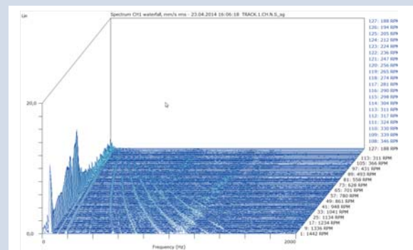
Tracking FFT waterfall plot
