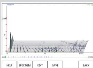
Tracking FFT waterfall plot
