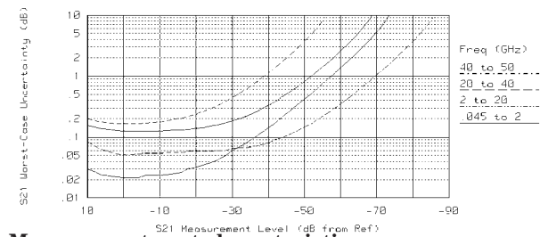
Measurement port characteristics
