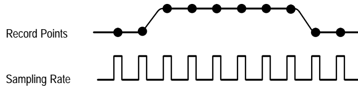
Figure 2-5: Real-Time Sampling
