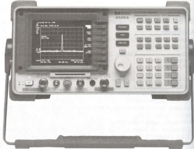
HP 8595A
