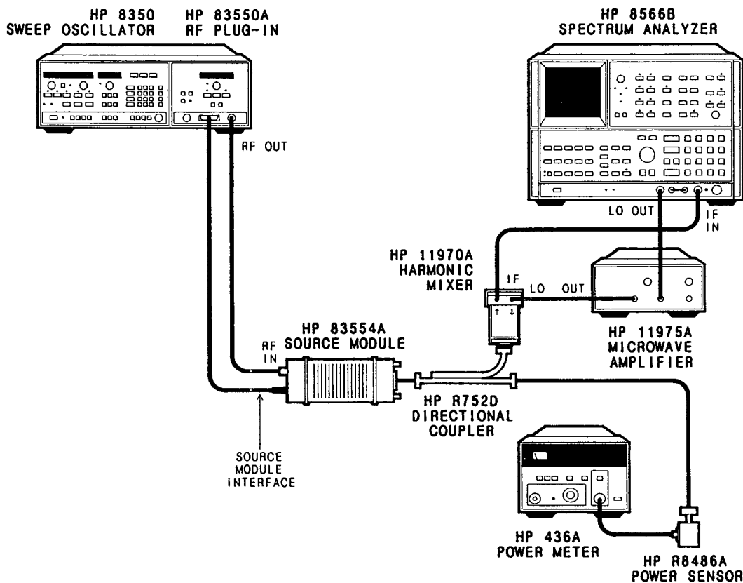
Figure 2-10. Spurious Signals Test Setup
