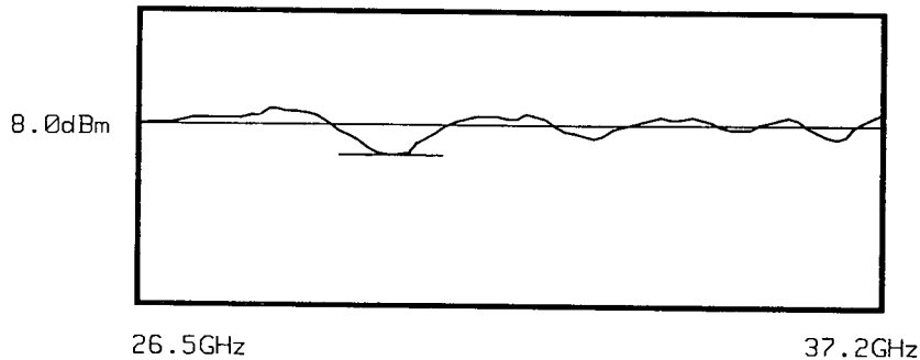
Figure 2-6. Minimum Power Point (26.5 to 37.2 GHz)
