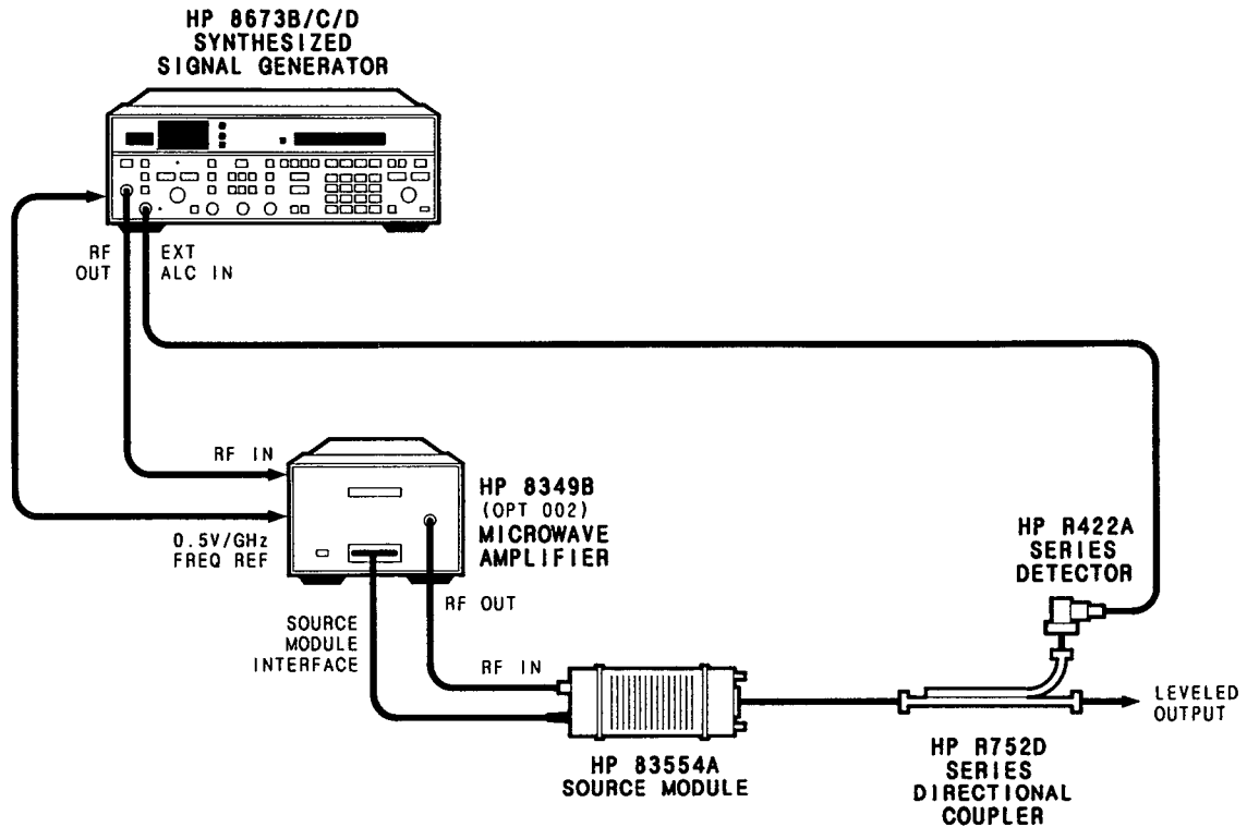
Figure 2-2. External Crystal Detector at the HP 83554A Source Module Output.
