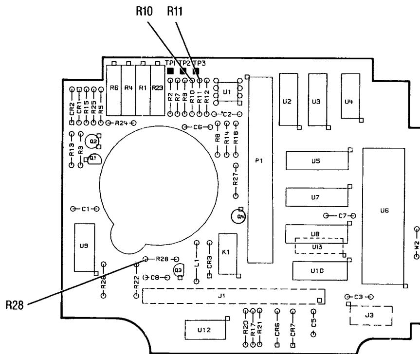
Figure 4. A2 Sub Panel Assembly, Component Locations.
