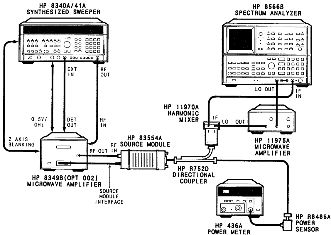
Figure 2-9. Spurious Signals Test Setup
