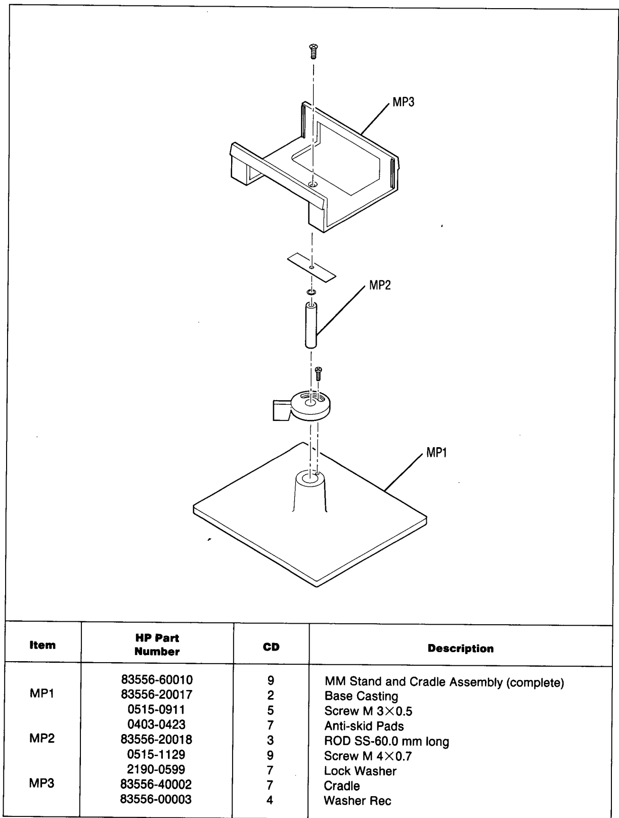
Figure 3-14. Source Module Stand, Exploded View
