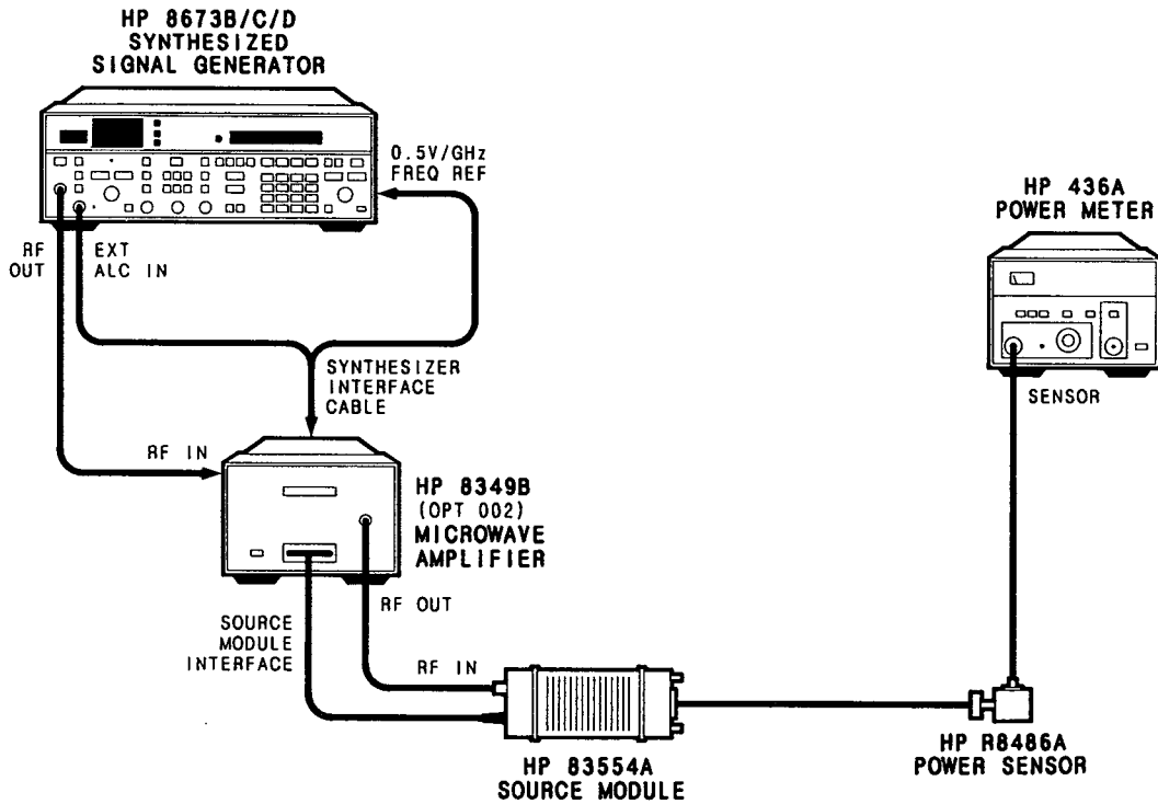
Figure 2-4. System Configuration
