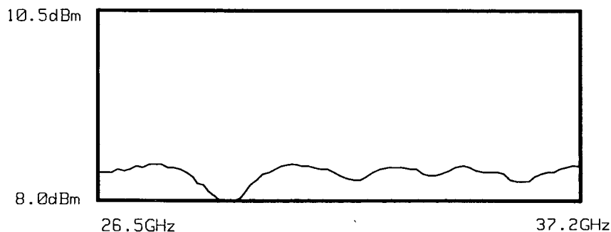
Figure 2-7. Power Flatness Response (26.5 to 37.2 GHz)
