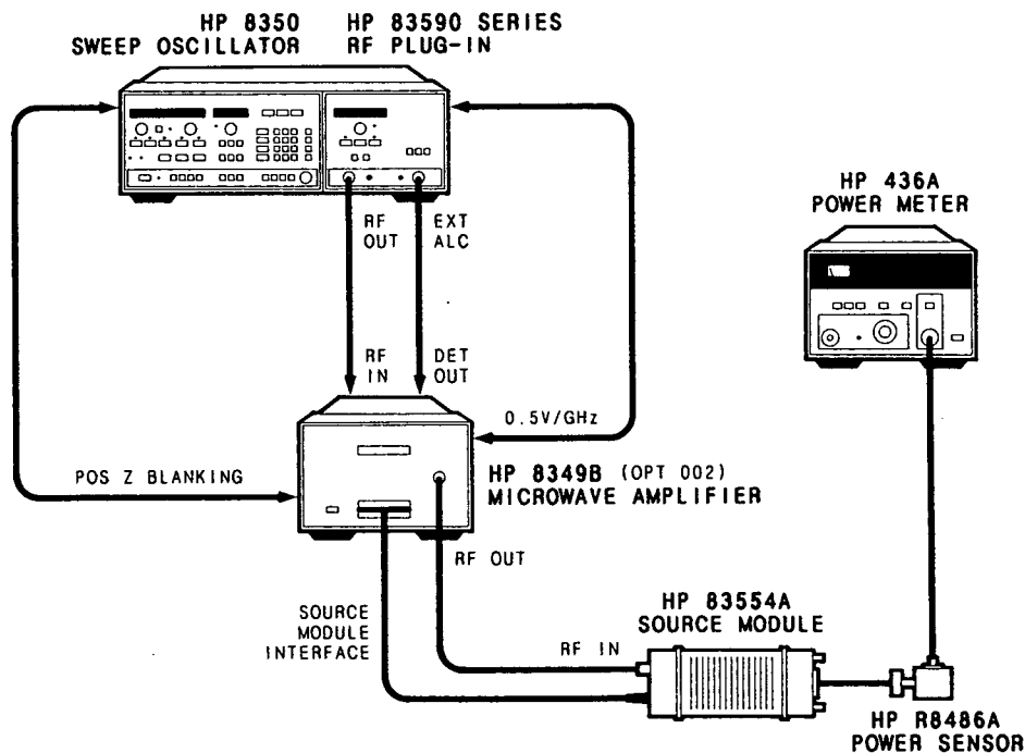
Figure 2-5. System Configuration
