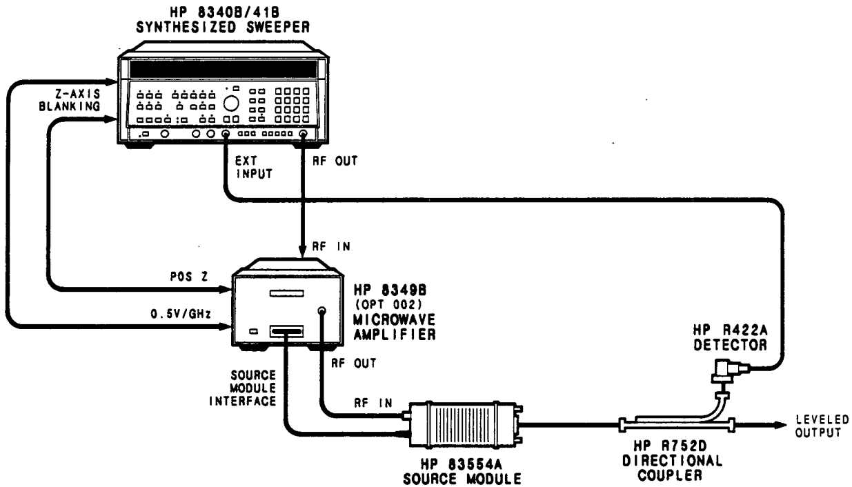
Figure 2-2. External Crystal Detector Leveling at the HP 83554A Source Module Output
