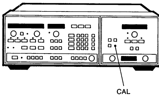
Figure 2-3. EXT CAL Adjustment Location
