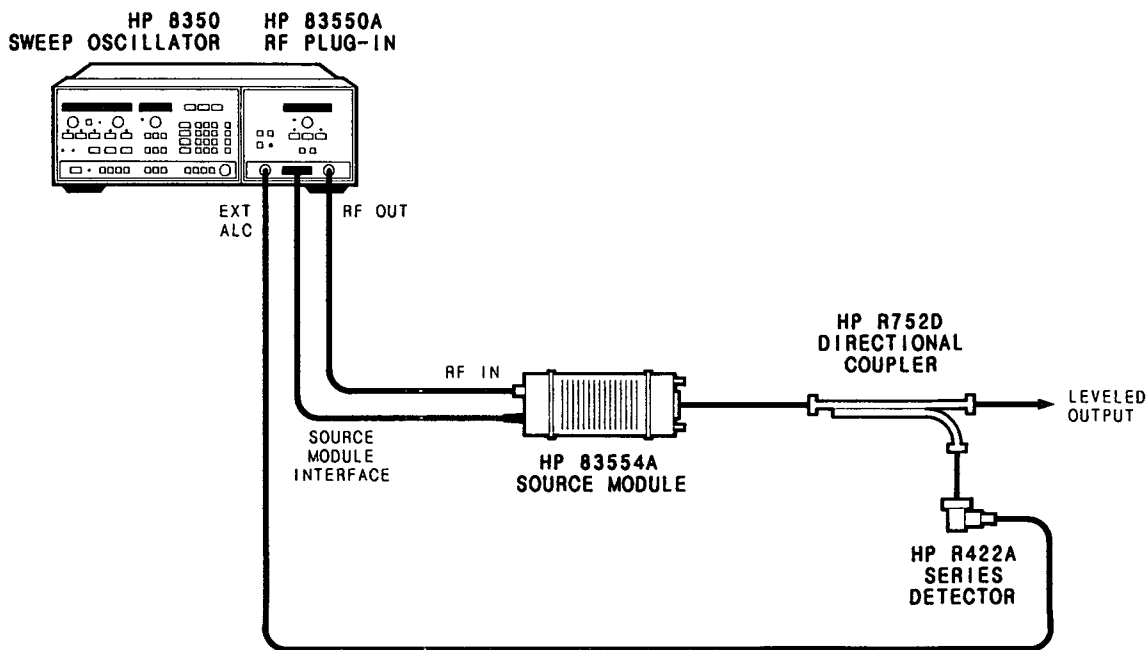
Figure 2-2. External Crystal Detector Leveling at the HP 83554A Output
