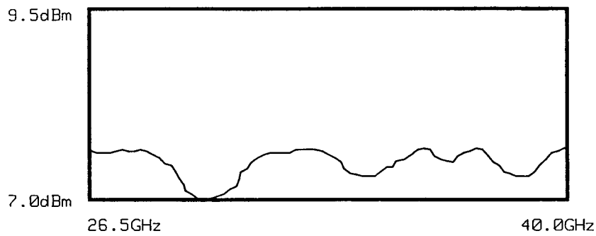
Figure 2-8. Power Flatness Response (26.5 to 40 GHz)
