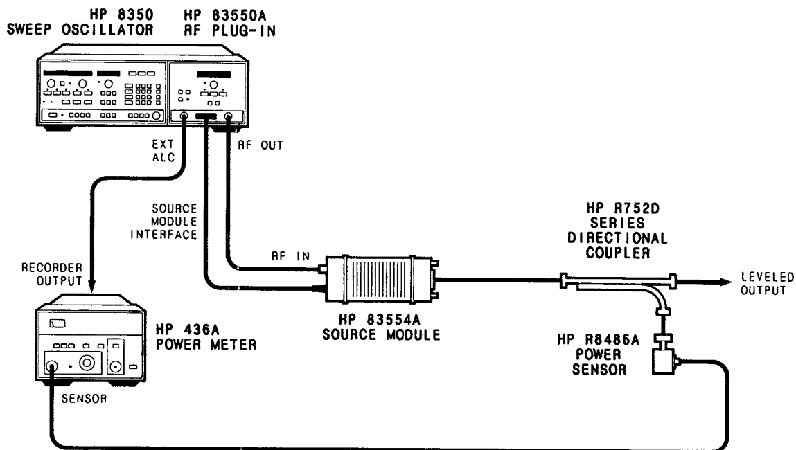
Figure 2-4. External Power Meter Leveling at the HP 83554A Output
