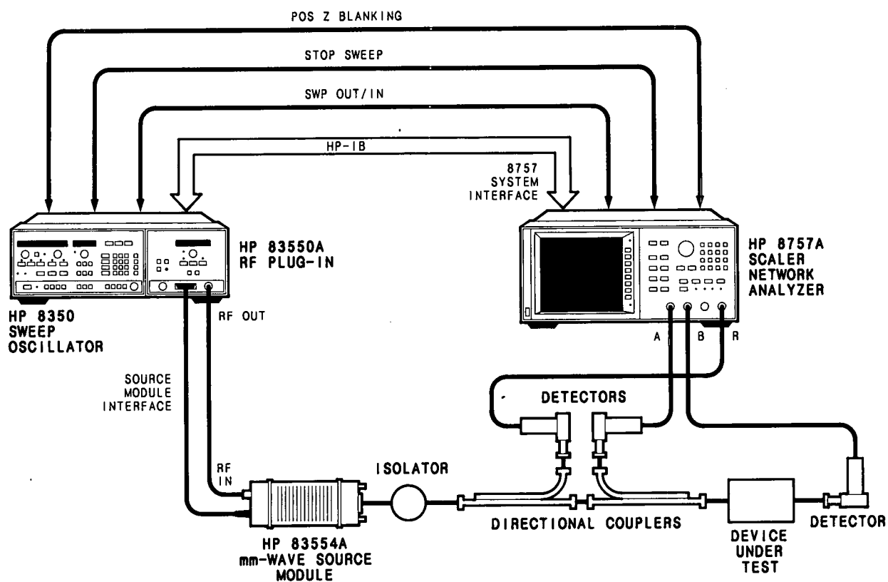
Figure 5. Typical Scalar Transmission and Reflection Millimeter-wave Measurement System
