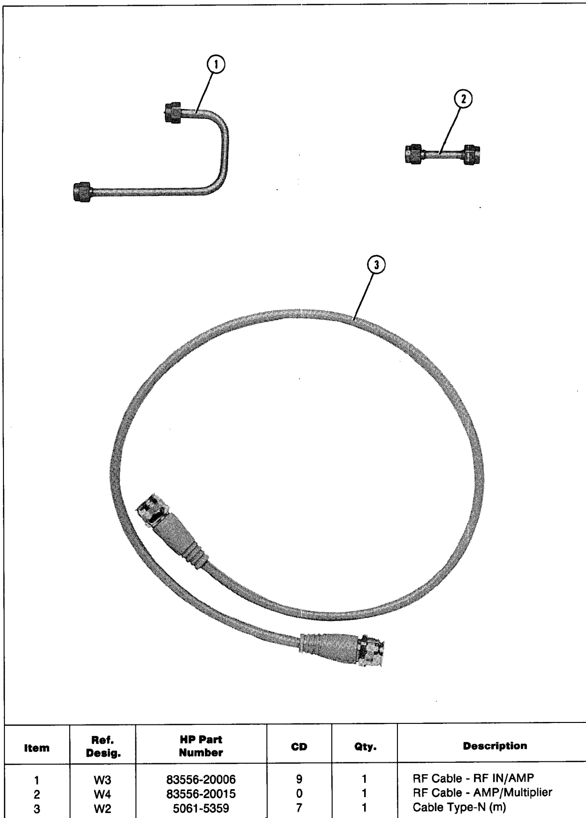
Figure 3-13. RF Cables Identification
