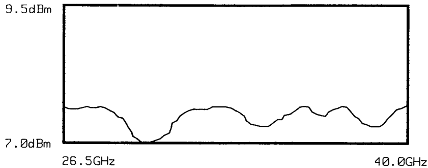
Figure 2-9. Power Flatness Response (26.5 to 40.0 GHz)
