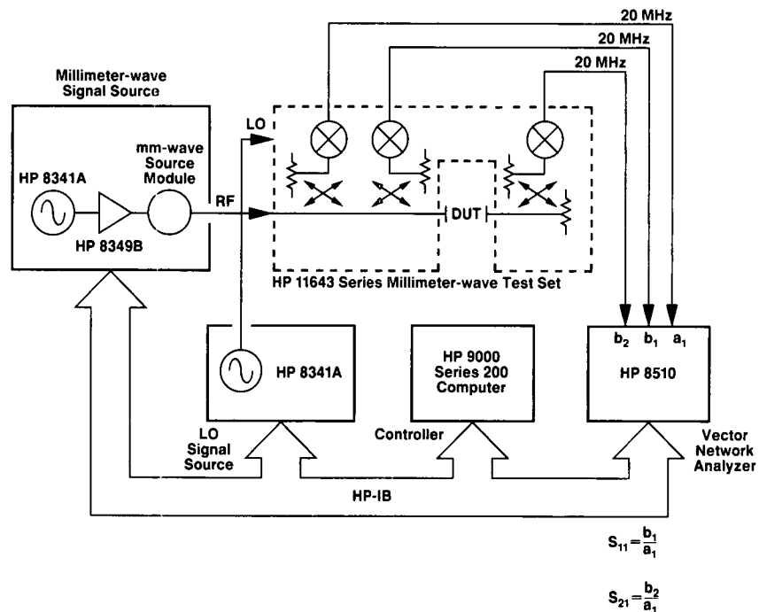
Figure 4. A Simplified Block Diagram of the Millimeter-wave Vector Network Analyzer
