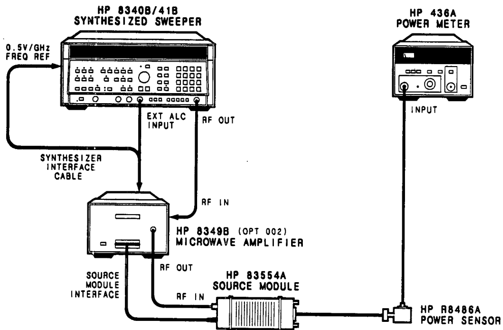
Figure 2-4. System Configuration
