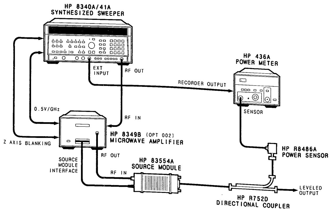
Figure 2-3. External Power Meter Leveling at the HP 83554A Source Module Output
