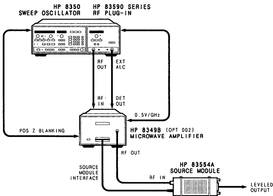
Figure 2-1. HP 83590 Series RF plug-in/83554A Source System Configuration
