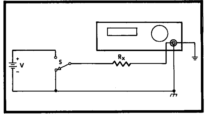
FIGURE 12. Volt-Ammeter Resistance Method.
