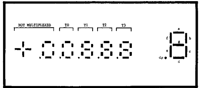
FIGURE 31. Digital Display.
