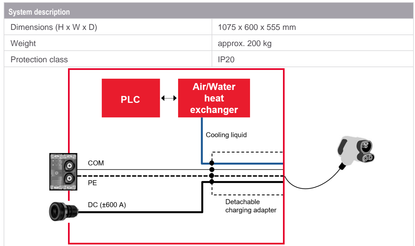
SL1048-CU1 – Scienlab Cooling Unit incl. liquid-cooled charging adapter
