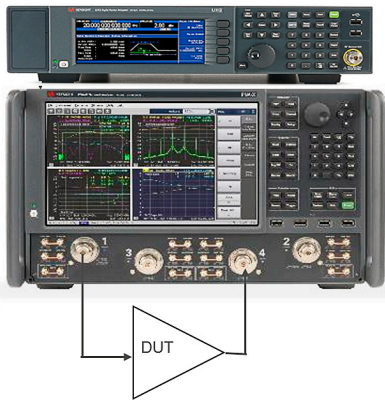
Classic NPR measurement with PNA/PNA-L and UXG
