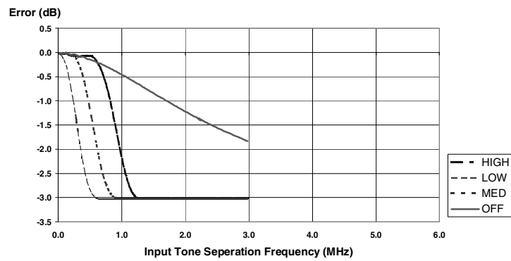
Figure 7 E9321A and E9325A Error in Peak-to-Average Measurements for a Two-tone Input (High, Medium, Low, and Off Filters)
