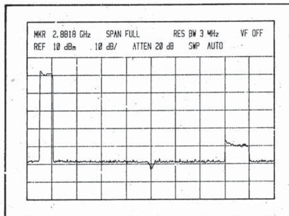
Figure 36. Oscillator Fundamental and Second Harmonic
