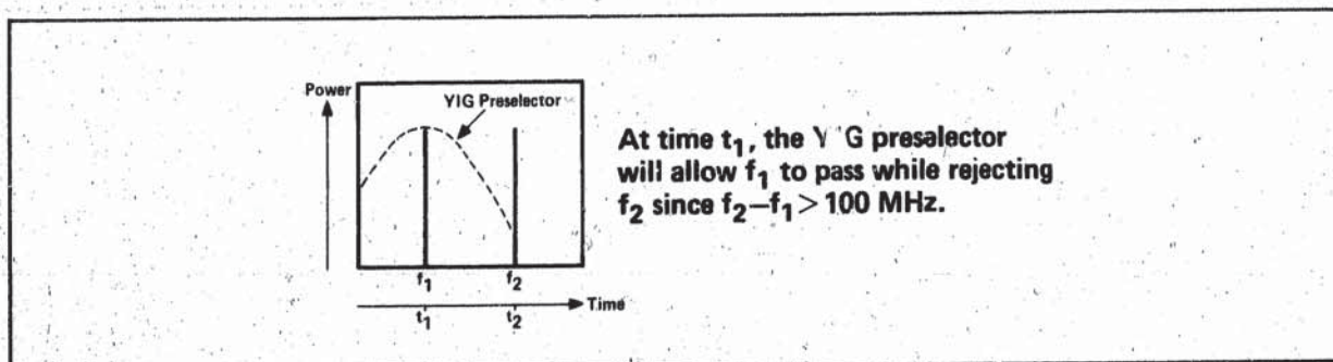
Figure 27. YIG Preselector Passband
