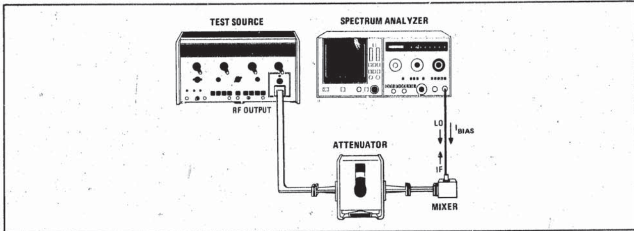
Figure 31. External Mixer Test Setup
