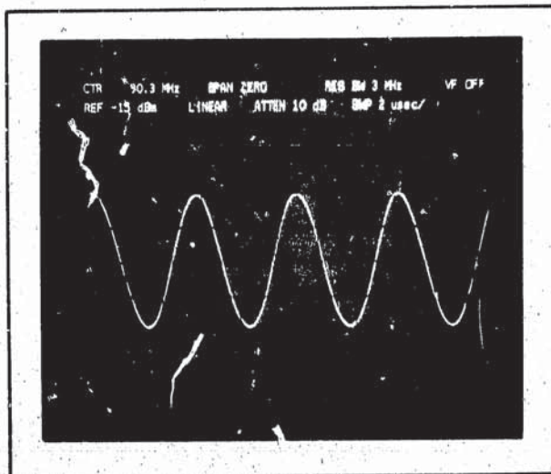
Figure 39. Demodulated AM Signal in ZERO SPAN
