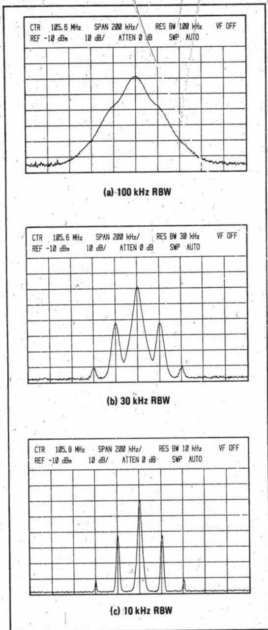
Figure 17. Resolving Modulation Sidebands
