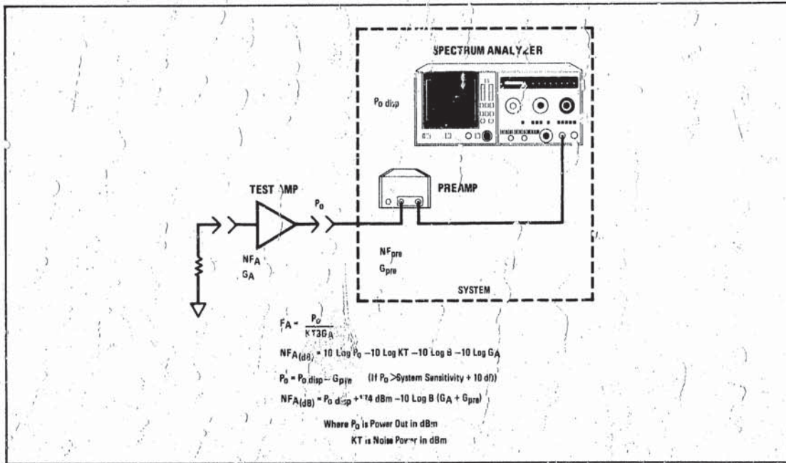
Figure 46. Measuring Noise Figure—Absolute Power Technique
