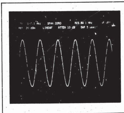
Figure 12. AM Carrier Demodulated in ZERO SPAN
