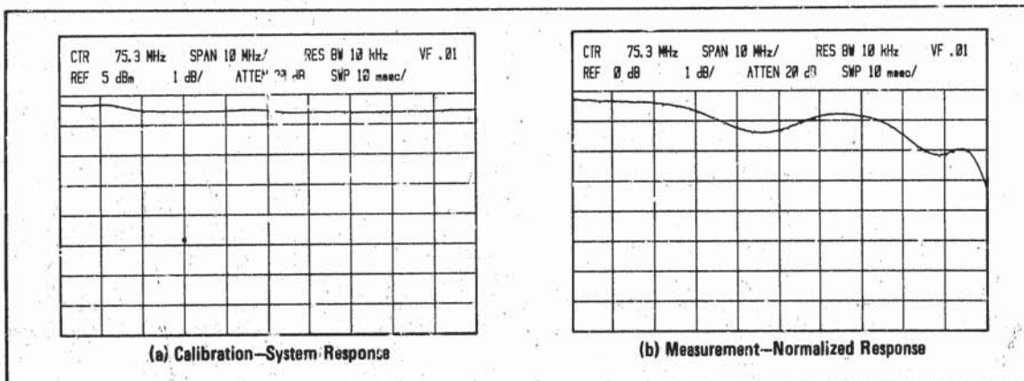
Figure 55. Normalization of Frequency Response
