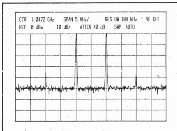
Figure 34. Two-Tone, Third Order Intermodulation Products
