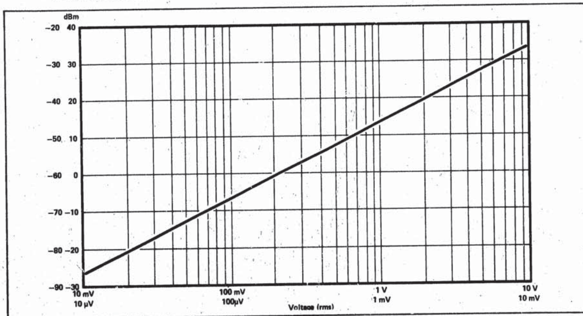
Figure 62. Conversion Chart - Converts from dBm to Voltage in 50Ω
