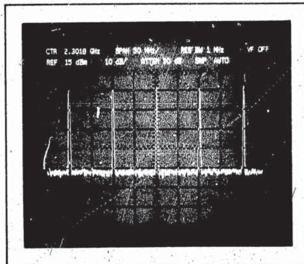
Figure 29. CRT Display with Character Annotation
