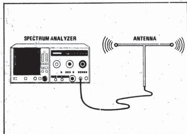
Figure 50. Field Strength Test Setup
