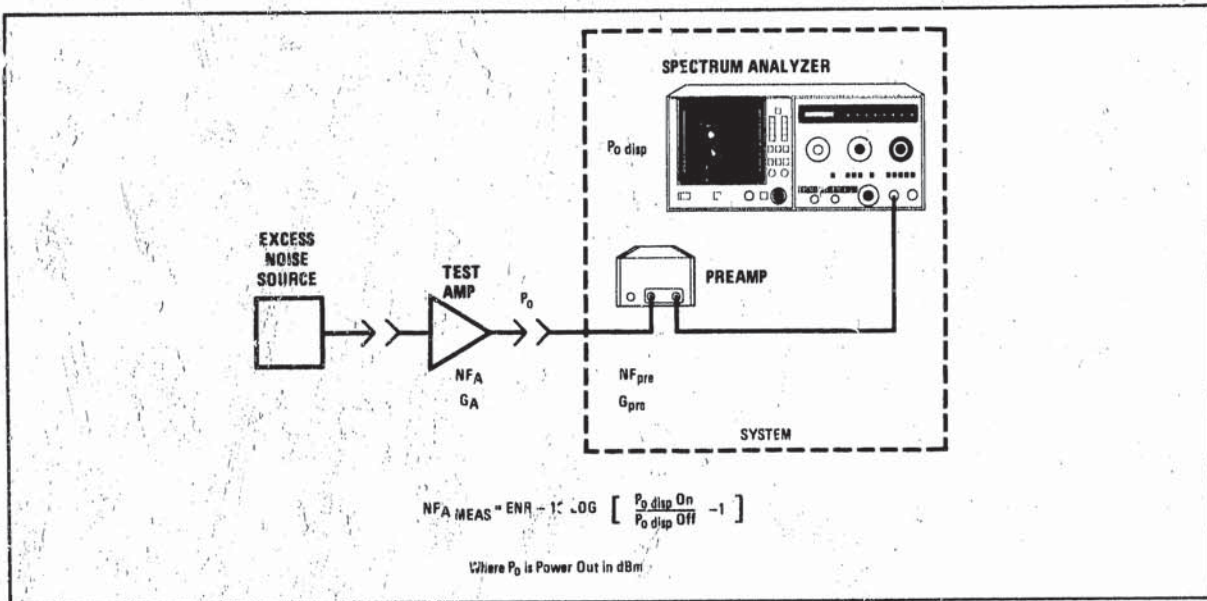
Figure 48. Measuring Noise Figure - Y Factor Technique
