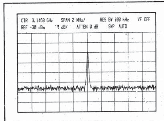
Figure 15. Analysis in PER DIV
