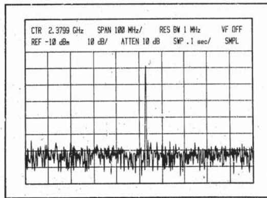
Figure 24. Sample Detection Mode
