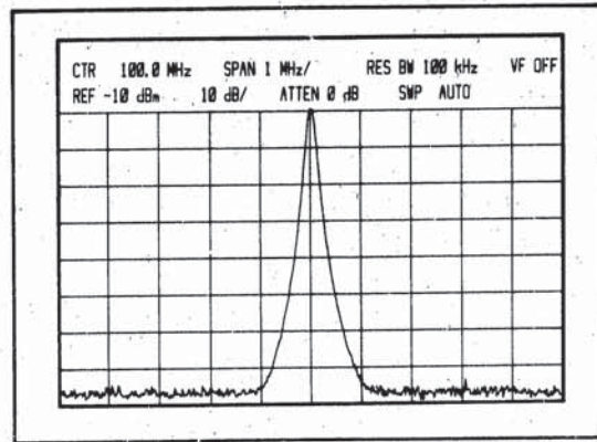
Figure 5. CAL OUTPUT Signal
