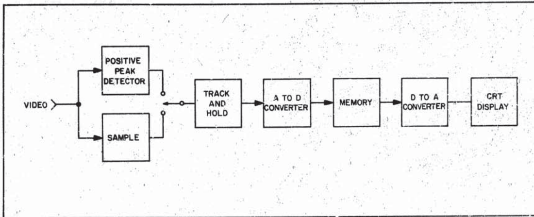
Figure 22. Detection Signal Flow
