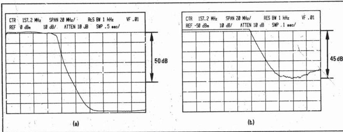
Figure 54. Low Pass Filter Measurement with 95 dB of Rejection
