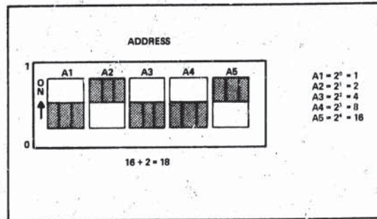
Figure 57. HP-IB Address Switch
