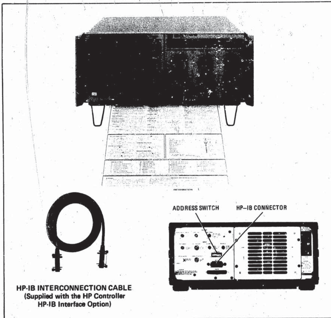
Figure 56. HP 8569A with HP-IB Interconnect Cable
