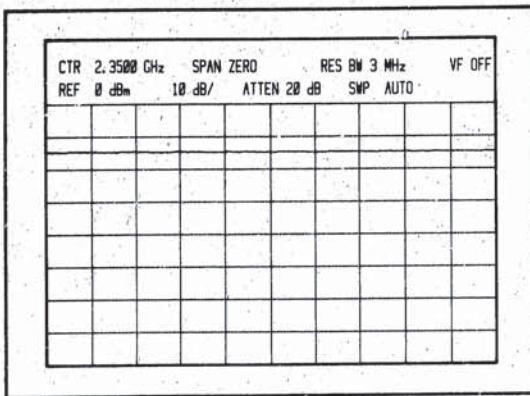
Figure 13. CW Measurement in ZERO SPAN
