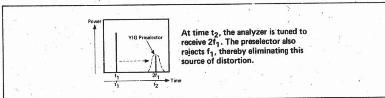
Figure 26. YIG Preselector Tuning
