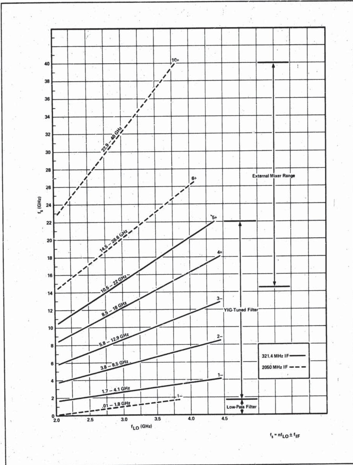
Figure 61. HP 8569A Tuning Curves
