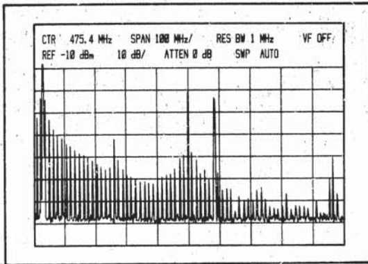
Figure 51. Radiated Interference
