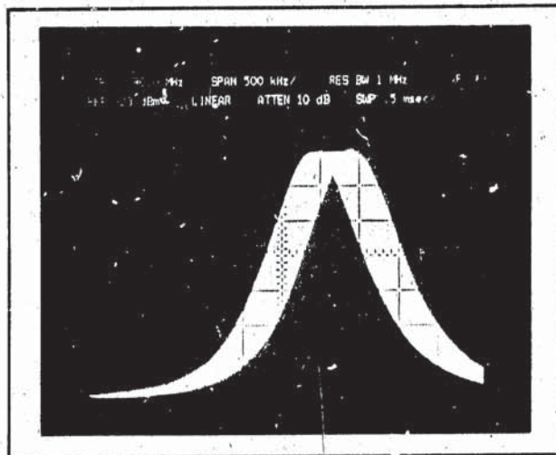
Figure 41. Slope Detection of FM Signal
