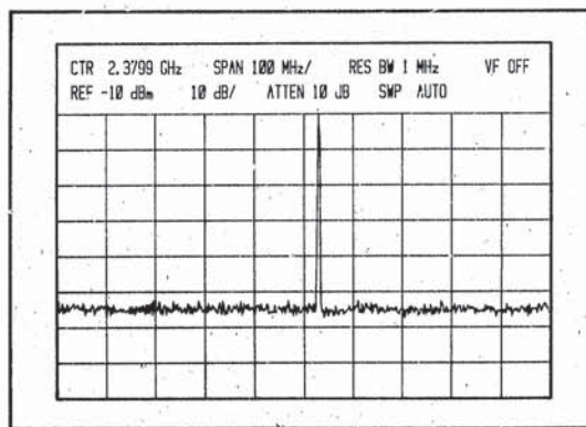
Figure 23. Normal Detection Mode
