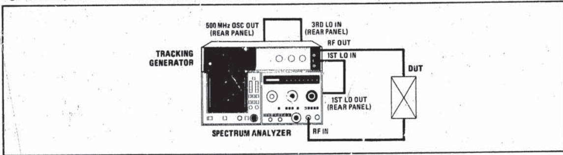
Figure 53. Swept Frequency Response Setup
