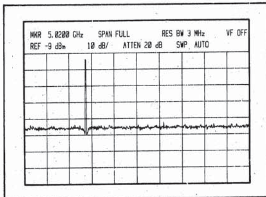
Figure 7. Tuning Marker in FULL BAND
