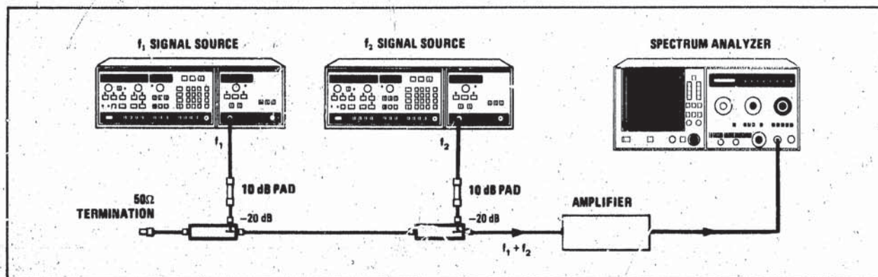
Figure 33. Two-Tone Test Setup
