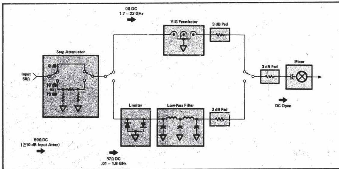
Figure 59. DC Block Diagram
