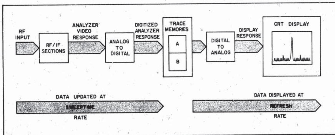
Figure 21. Data Acquisition and Transfer
