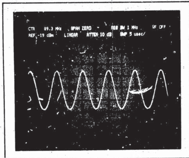
Figure 42. Demodulated FM Signal in ZERO SPAN
