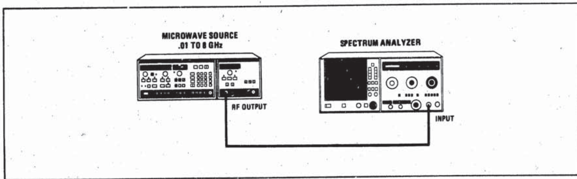
Figure 6. Microwave Source Test Setup
