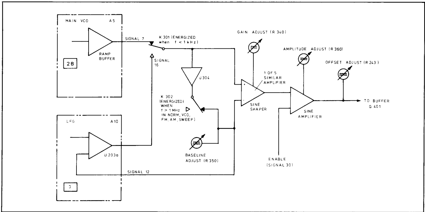
Figure 8-3-12. Sine Operation
