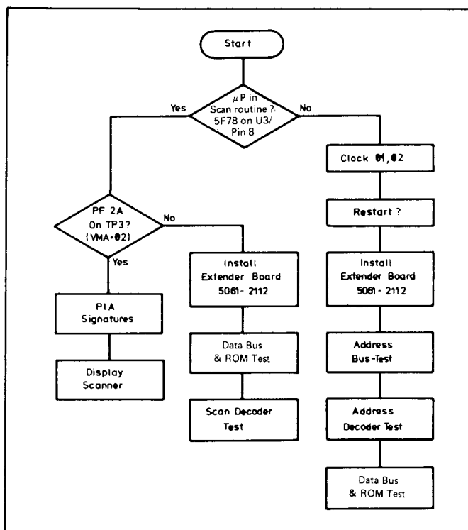
Figure 8-5-6. Flow chart
