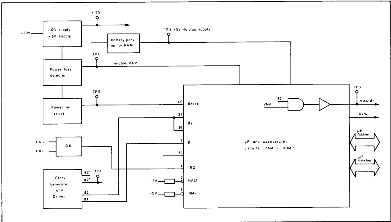
Figure 8-5-3. Microprocessor pre-conditions
