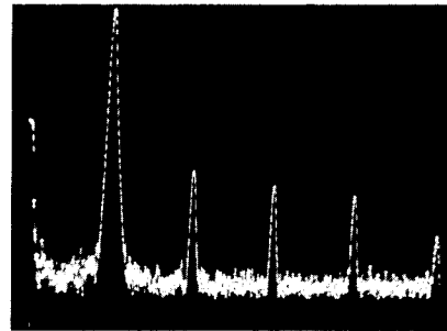
Figure 5-5. Sine Distortion Adjustment: 9.999 kHz
