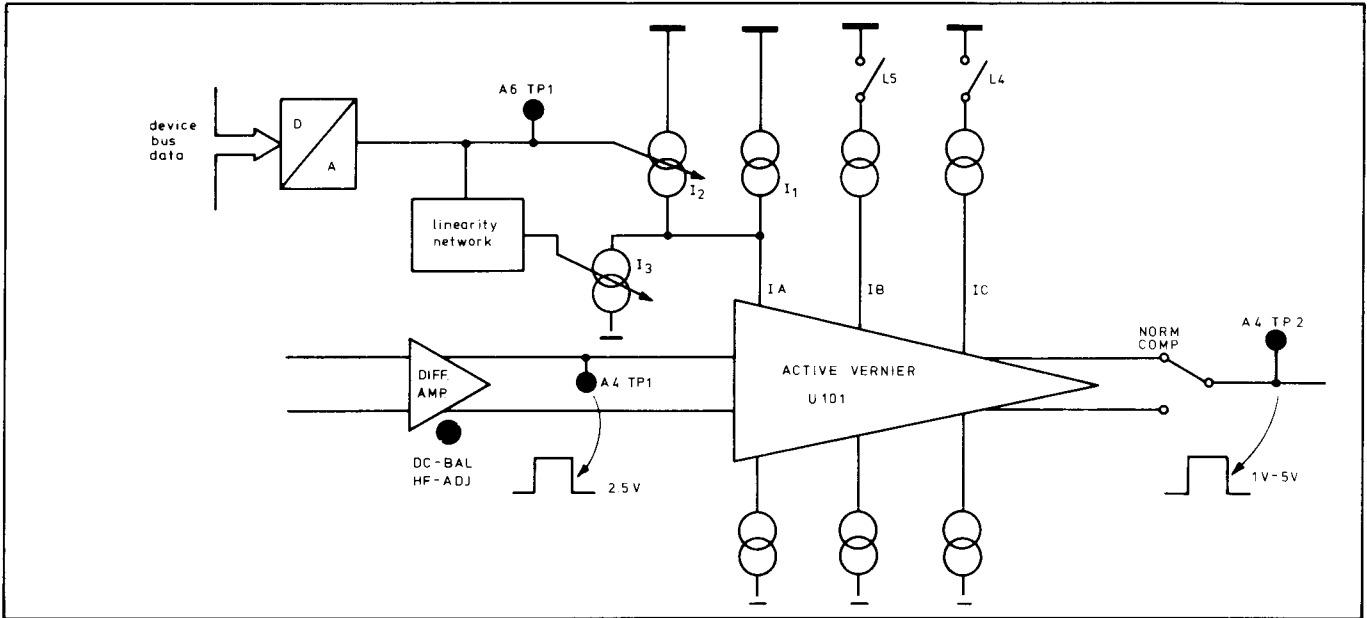
Figure 8-4-9. Active Vernier
