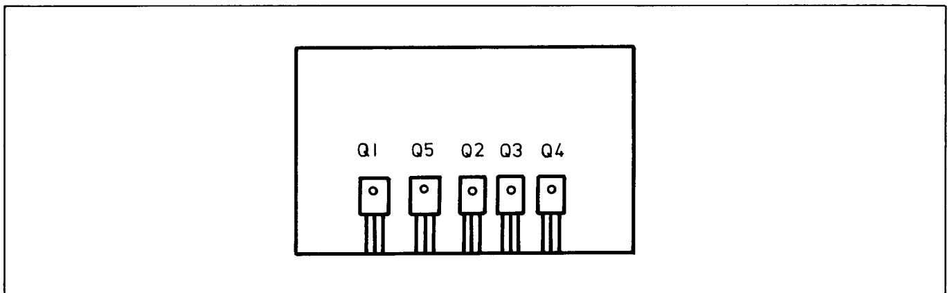
Figure 8-6-4. Heat-sink rear-view
