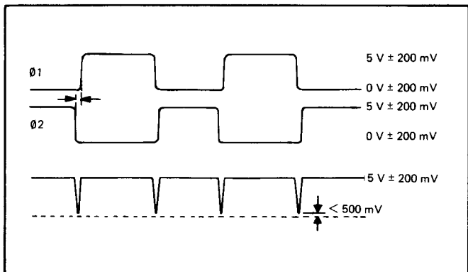
Figure 8-5-4. \mu\text{P} clock
