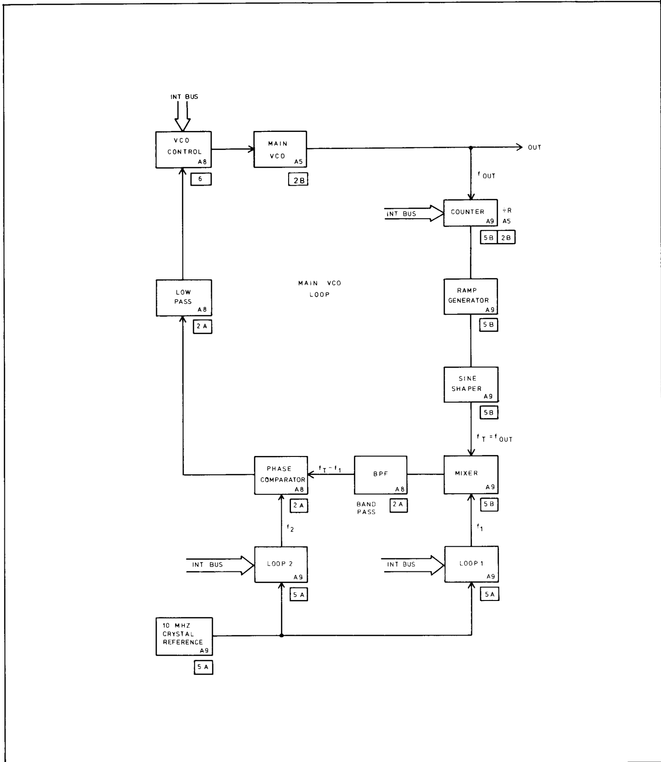
Figure 8-3-7. Frequency Synthesis in the 8165A
