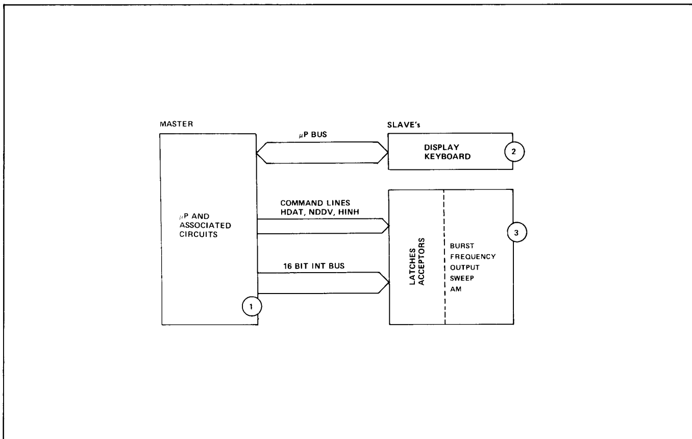
Figure 8-1-2. Categories of 8165A Malfunction
