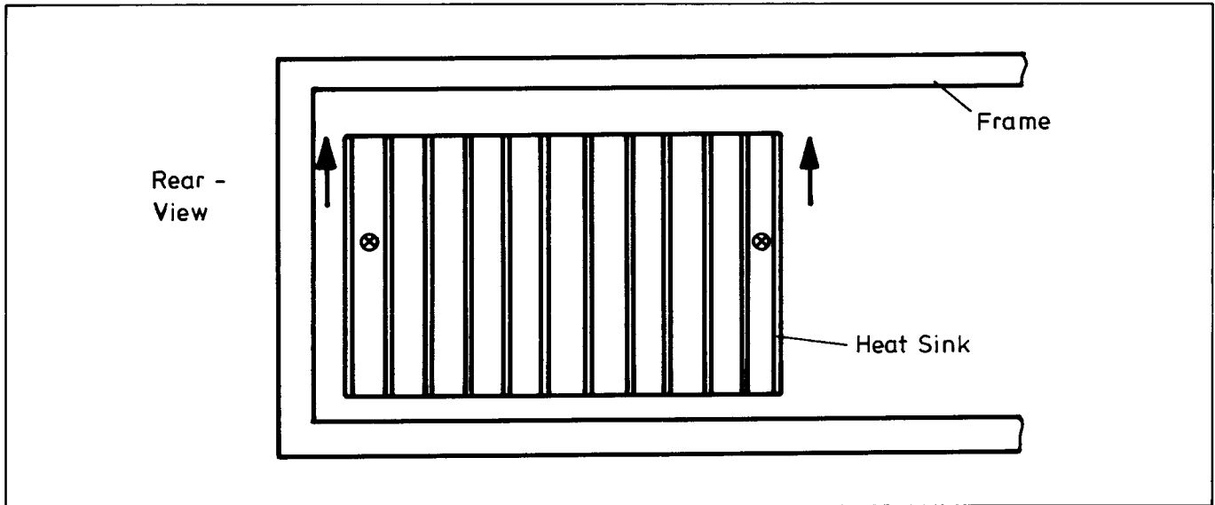
Figure 8-6-3. Heat-sink dis-assembling
