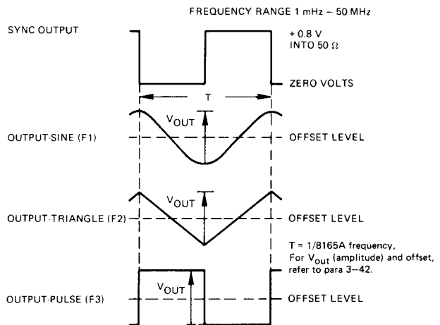
Figure 3-2 Normal Mode (50 % duty cycle/symmetry)
