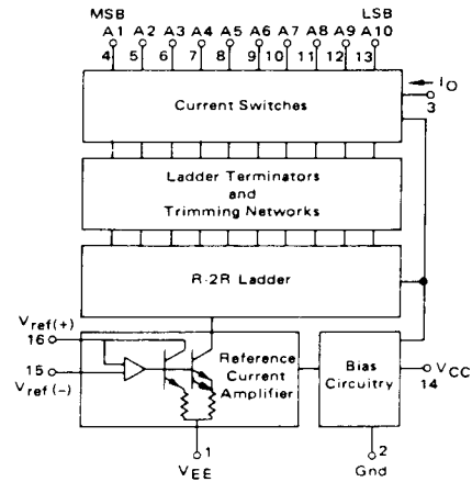
FIGURE 2 - TEN-BIT D/A CONVERTER BLOCK DIAGRAM
