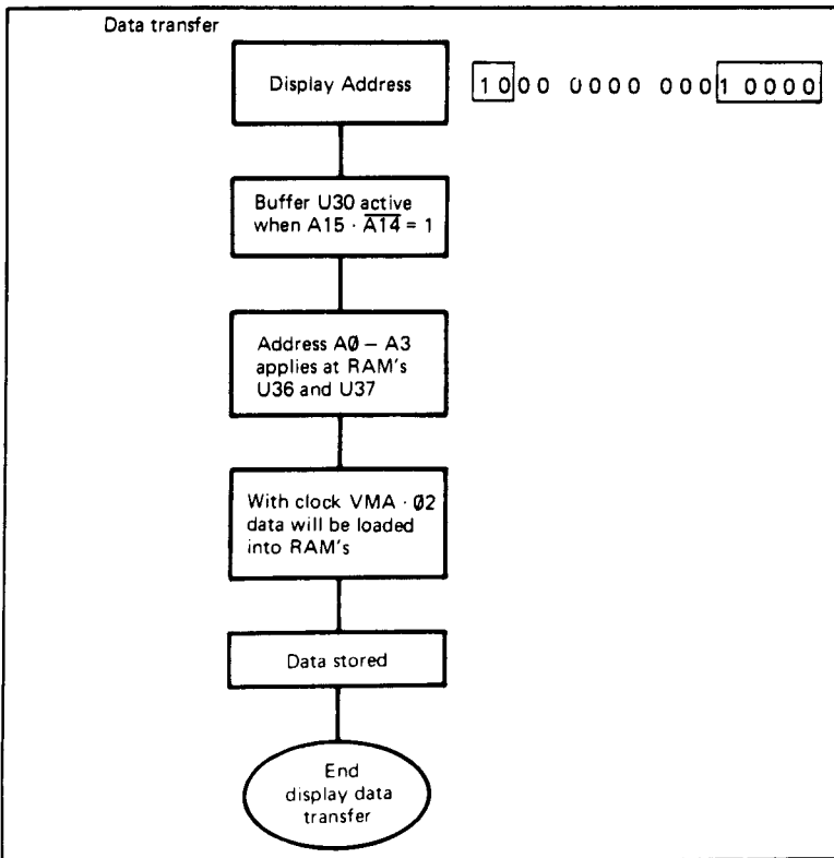
Figure 8–5–10. Display flowchart
