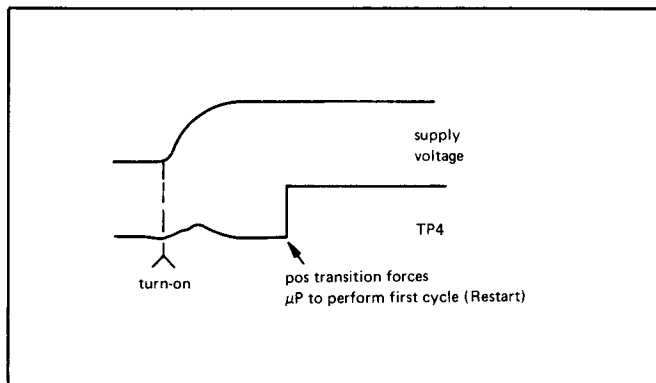
Figure 8-5-5. Power on/re-start
