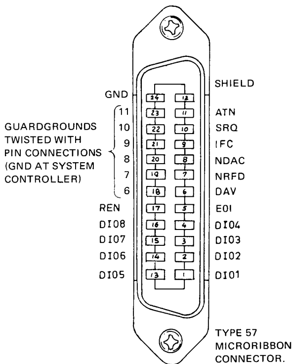
Figure 2-3. HP-IB Connector
