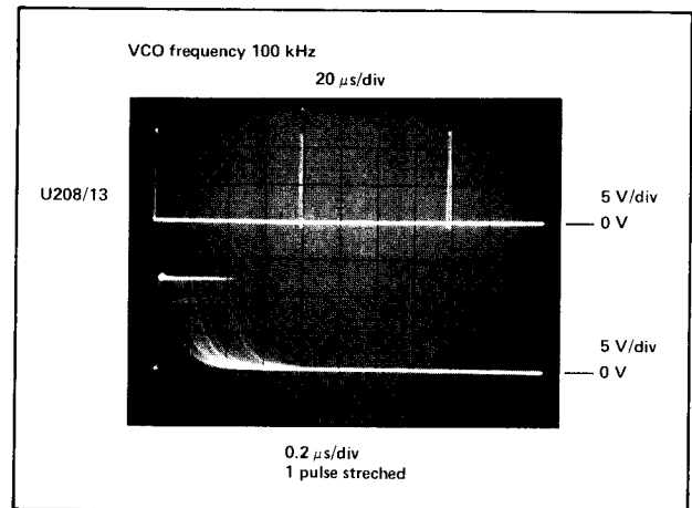
Figure 8-3-28. Waveform loop 1
