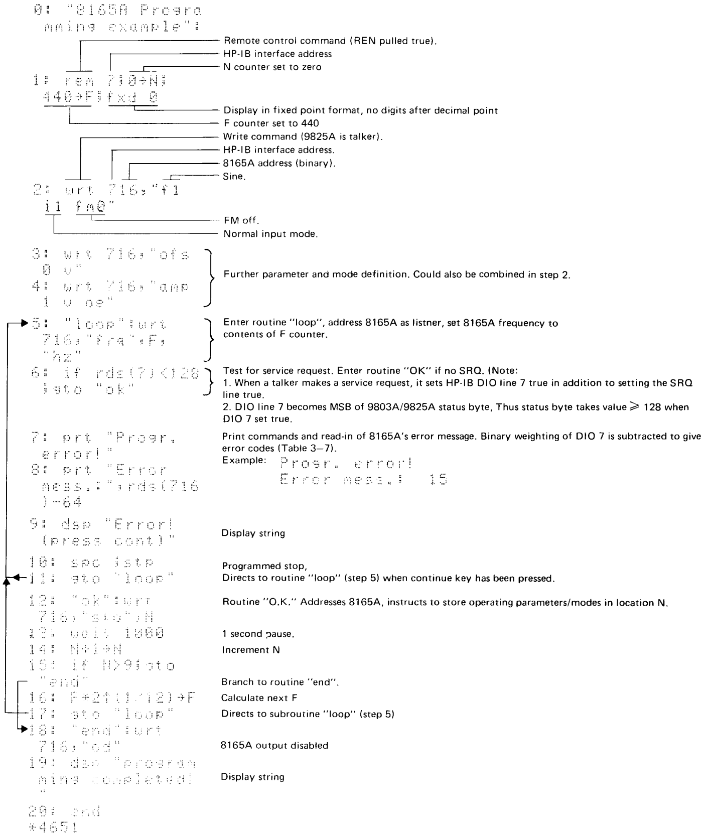
Figure 3-16. Program Example
