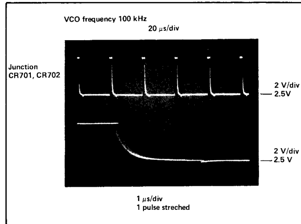
Figure 8-3-29. Waveform loop 2
