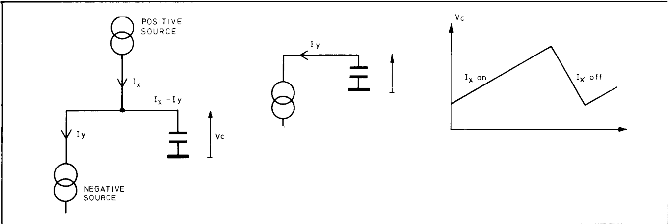
Figure 8-3-2. Ramp Generation
