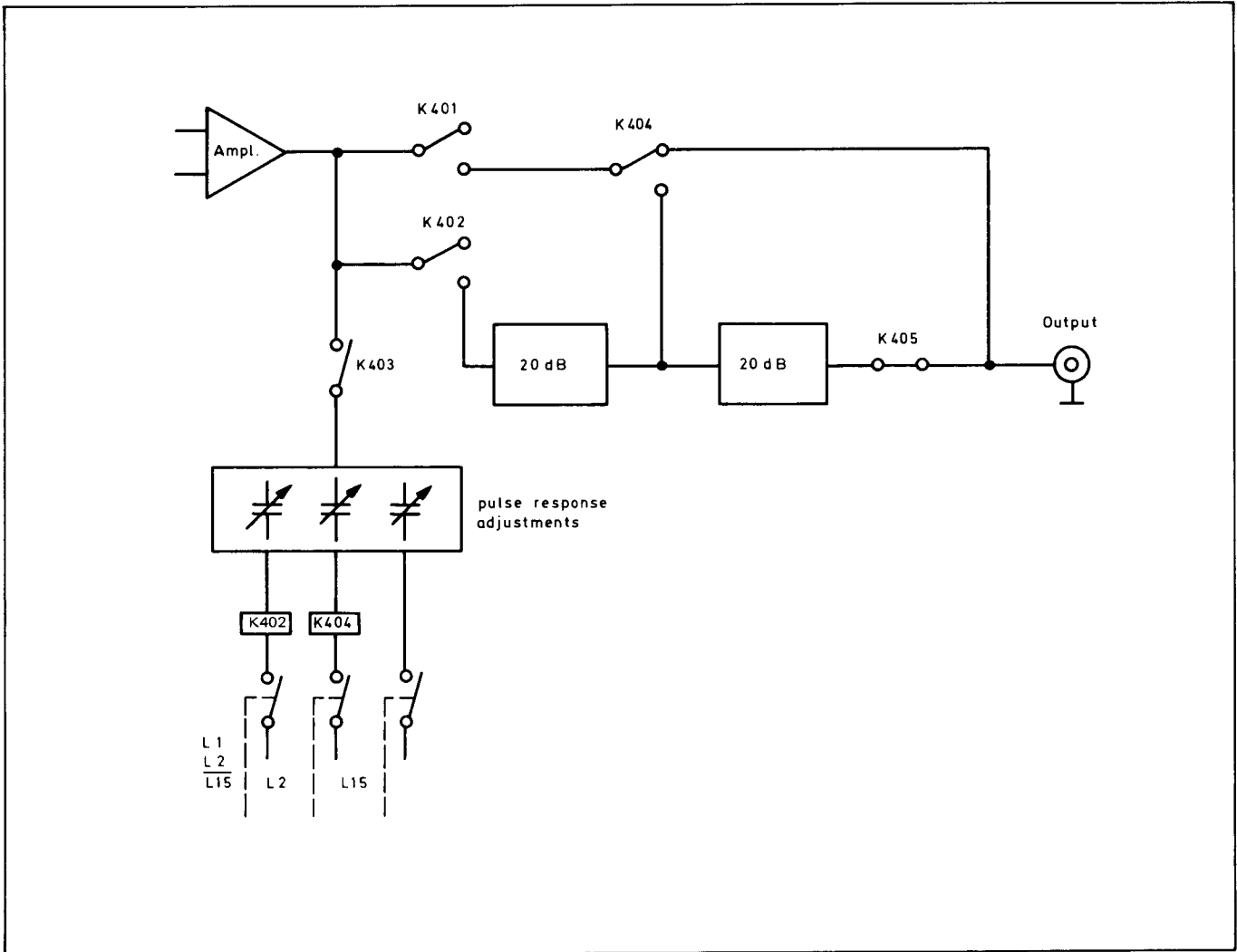
Figure 8-4-7. Attenuator ranges
