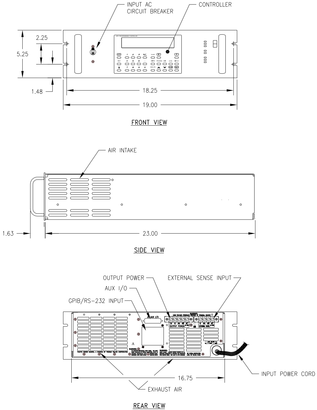
FIGURE 2.2.1 OUTLINE DRAWING, MODELS 115, 120, 315, & 320-ASX
