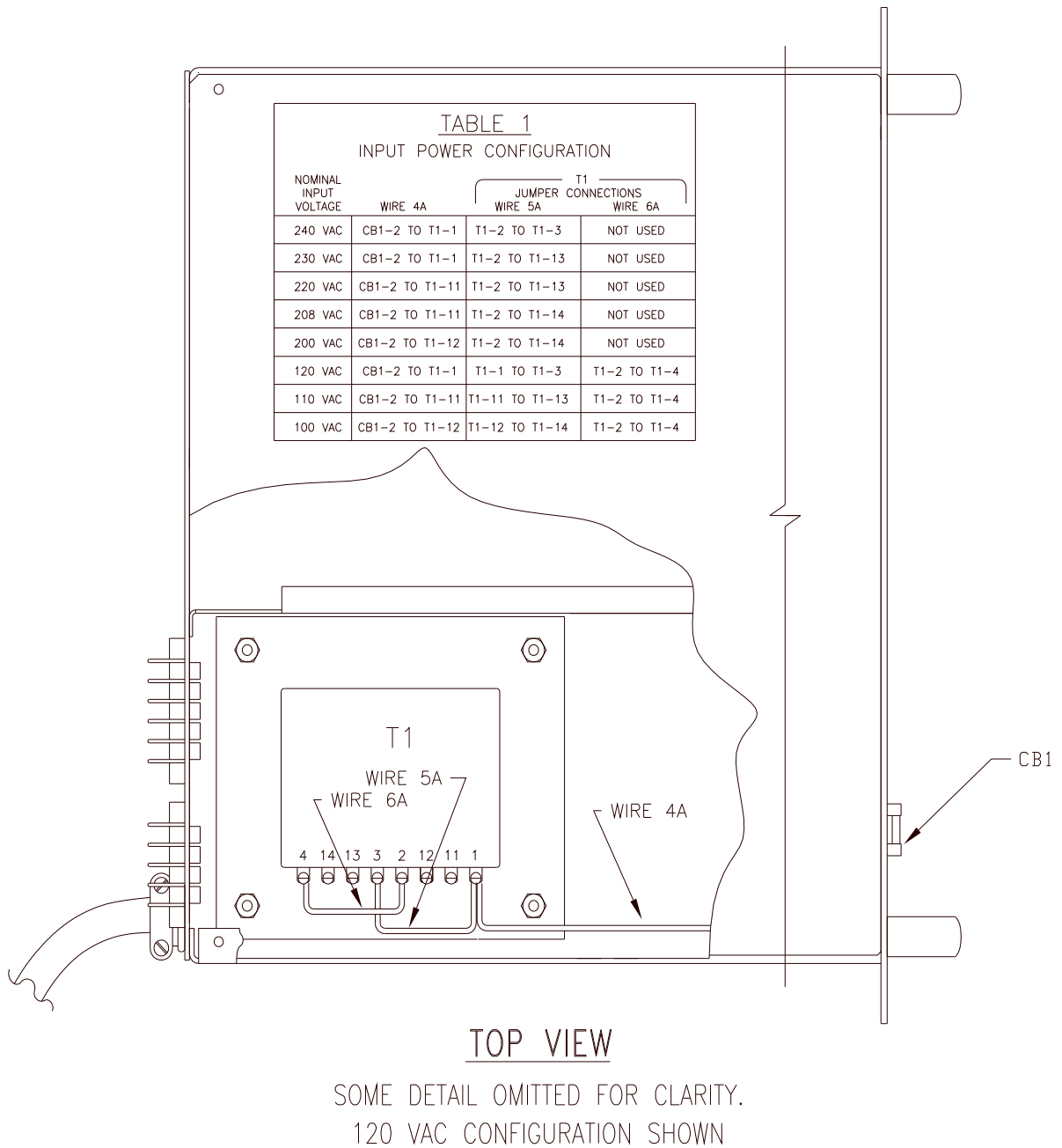
FIGURE 3.3.2 MODELS 120-ASX AND 320-ASX INPUT VOLTAGE CONFIGURATION
