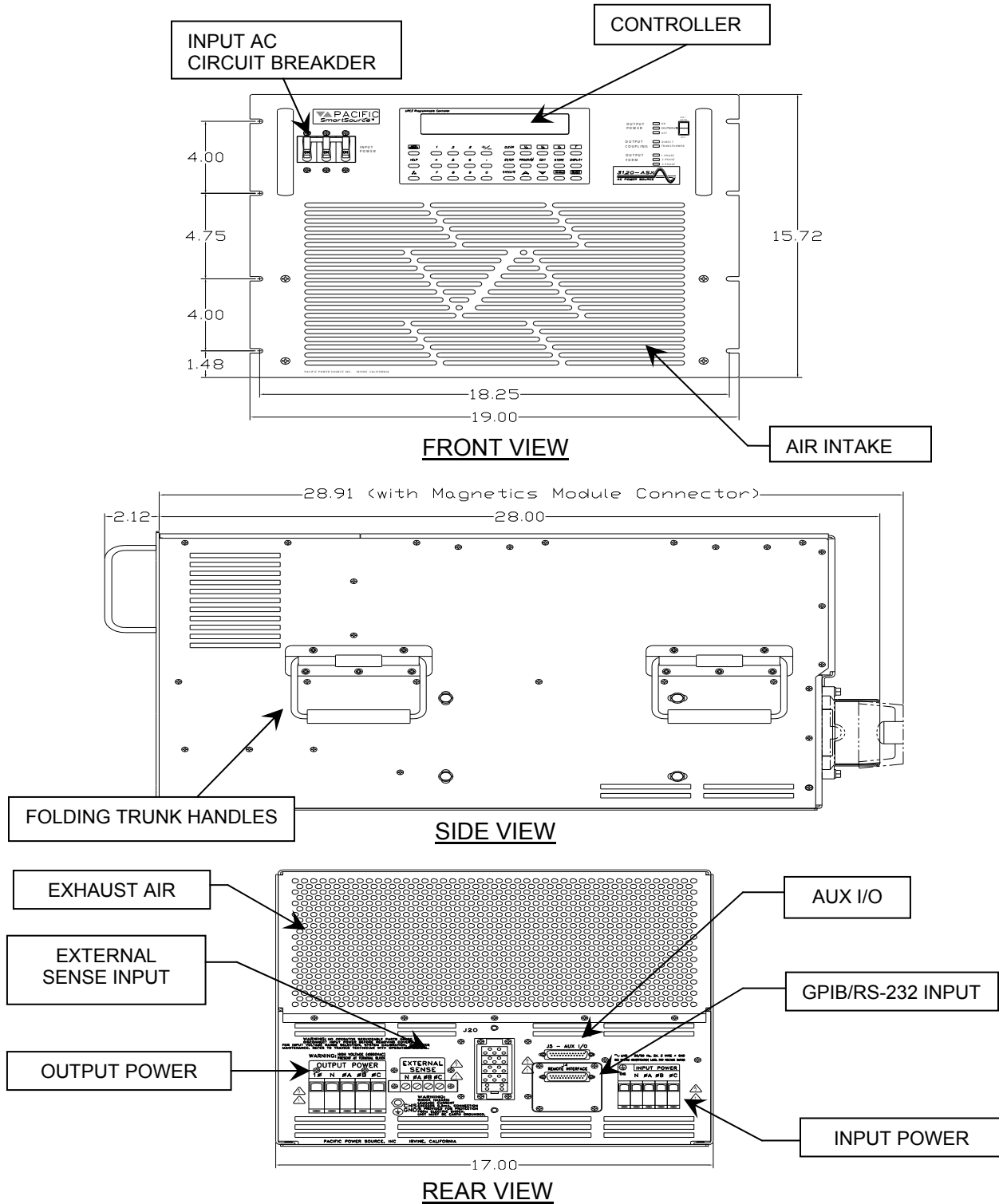
FIGURE 2.2.3 OUTLINE DRAWING, MODEL 3120-ASX
