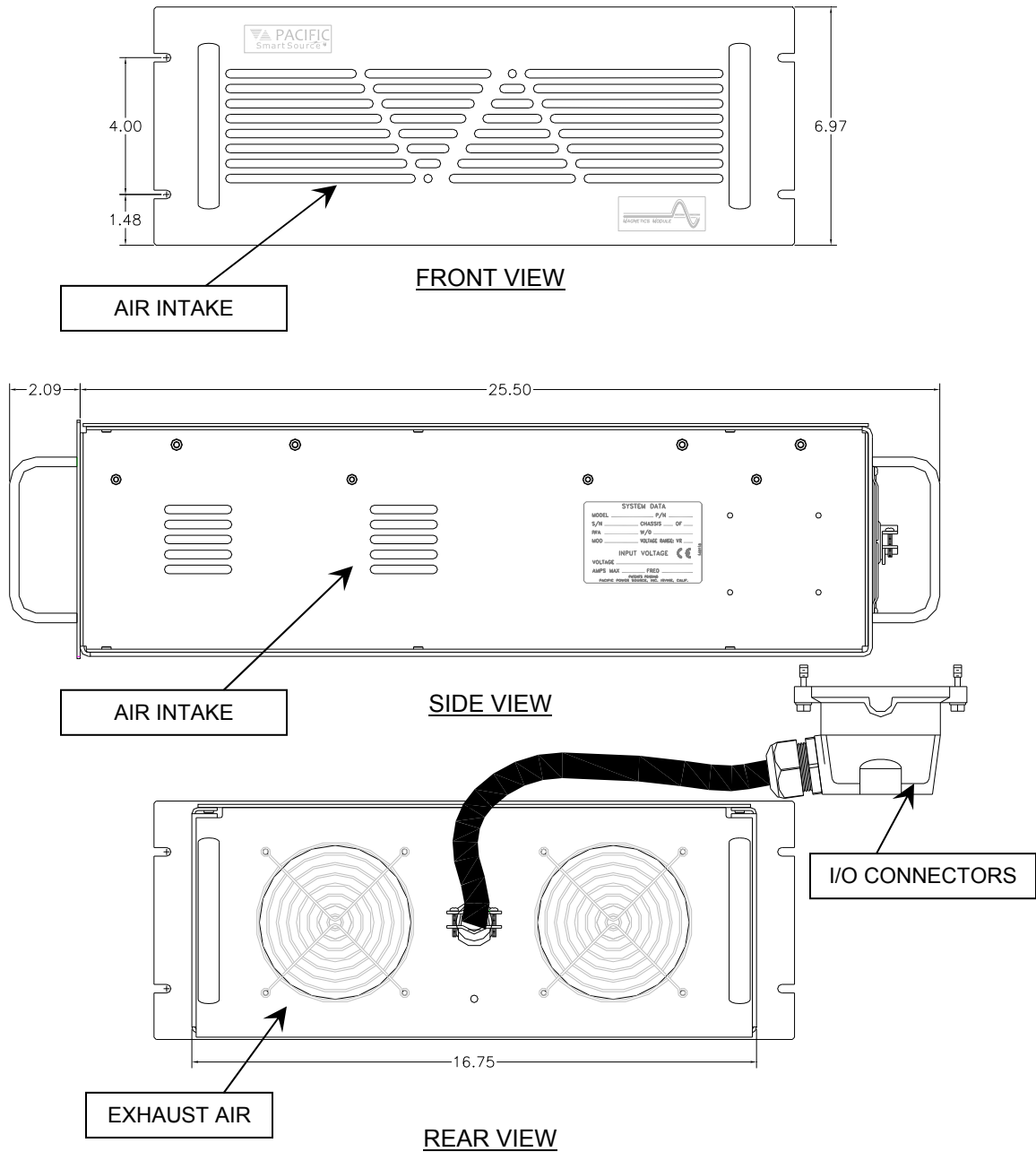
FIGURE 2.2.5 OUTLINE DRAWING, MODEL 3120-ASX MAGNETICS MODULE
