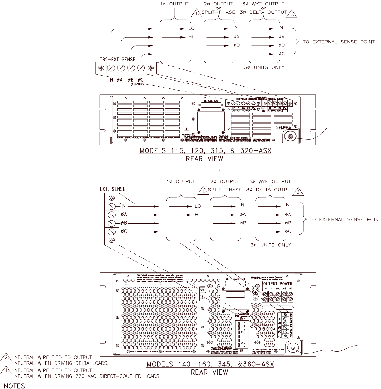
FIGURE 3.8.1 MODELS 115, 120, 140, 160, 315, 320, 345, & 360-ASX EXTERNAL SENSE CONNECTION
