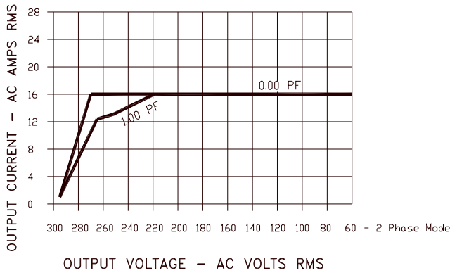
RATING CURVE 2 PHASE MODES
