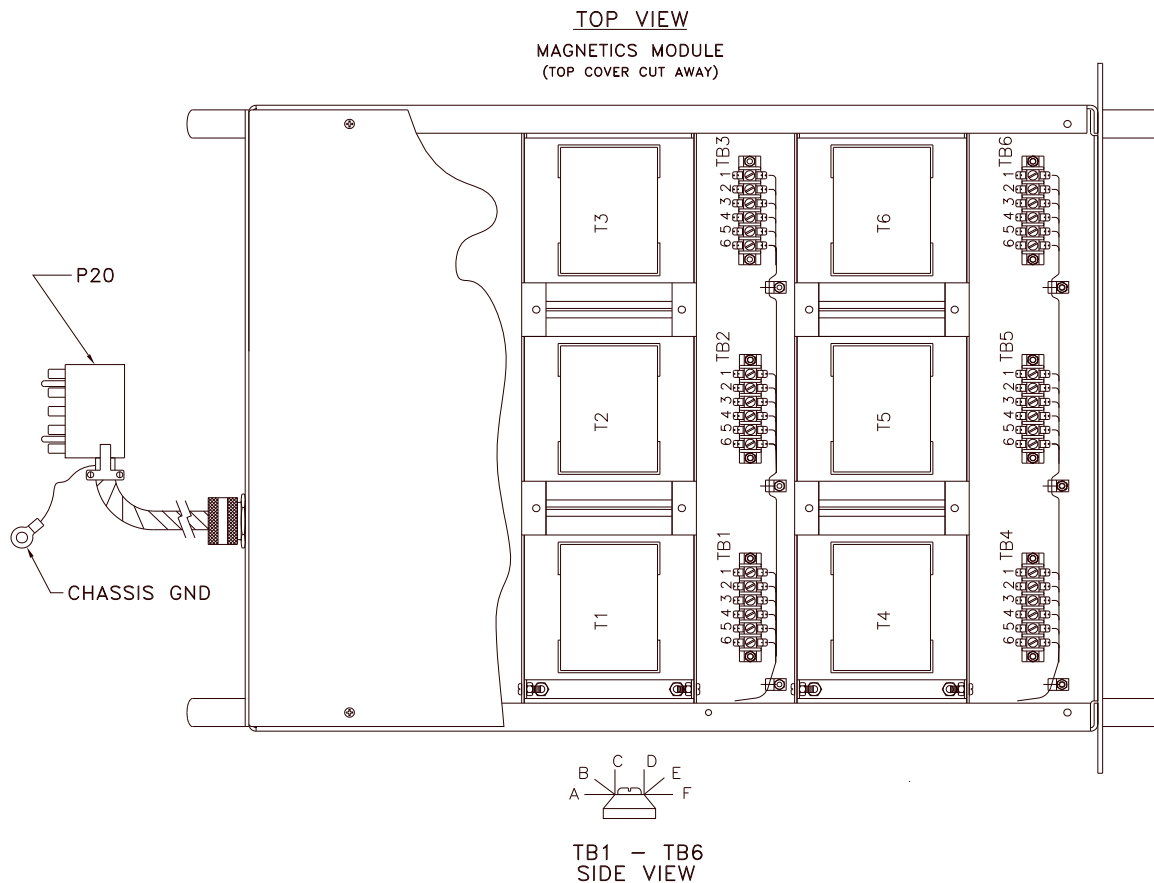
FIGURE 3.2.3 MODELS 140, 160, 345, & 360-ASX OUTPUT VOLTAGE RANGE CONFIGURATION
