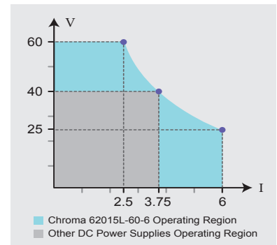
Autoranging Output
