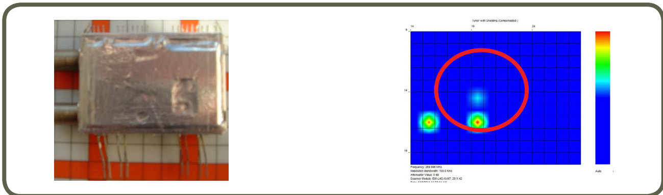
Fig. 8: Close-up of shielded board shown in Fig. 6.
