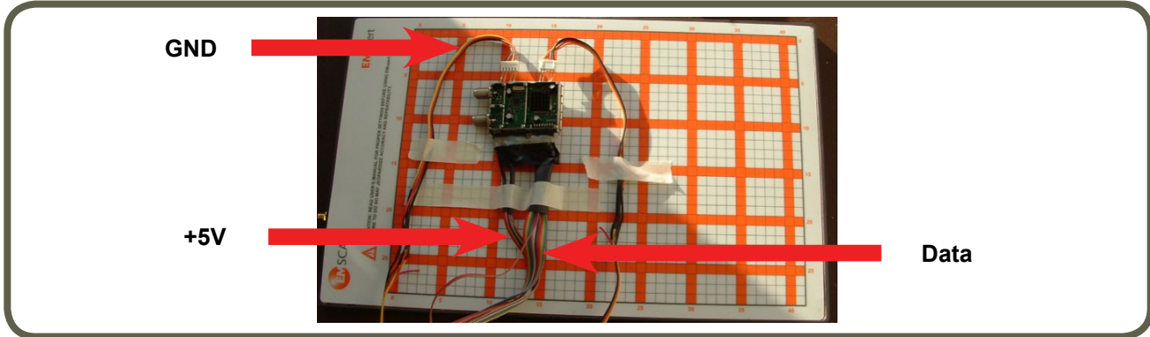
Fig. 5: Satellite Demodulator positioned on patented scanner.
