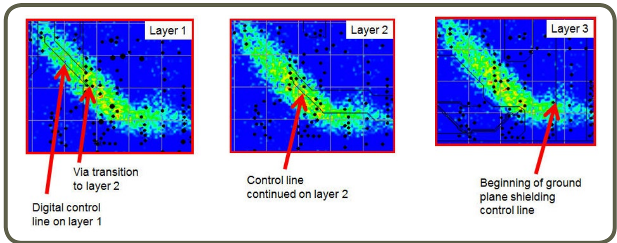
Fig. 16: Spatial Scan results of the PCB by EMxpert ERX+
