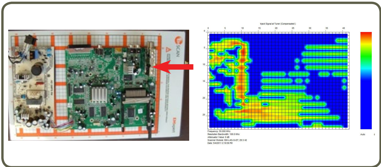
Fig. 15: EMxpert spatial scan at 50MHz with noise injection at right edge of board.
