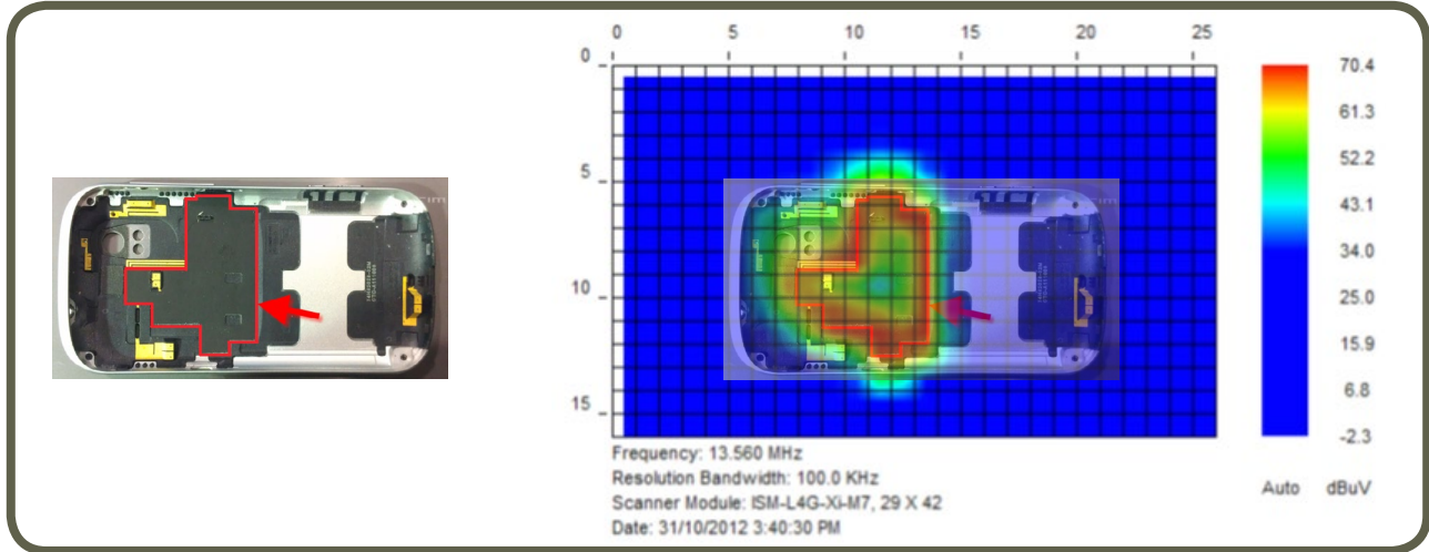
Fig. 19: Spatial Scan of the smart phone at 13.560 MHz
