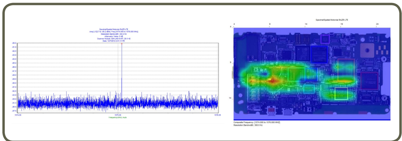
Fig. 20: Spectral Scan (left) and Spatial Scan (right) of the cellphone
