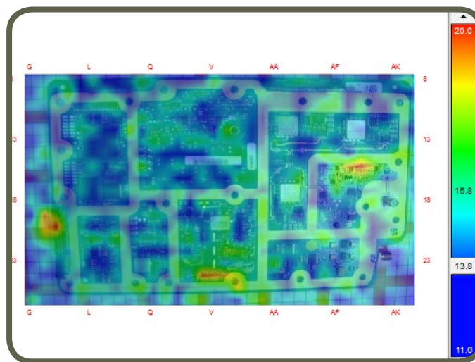
Fig. 22: Spatial Scan of the Bad Board at the IF frequency
