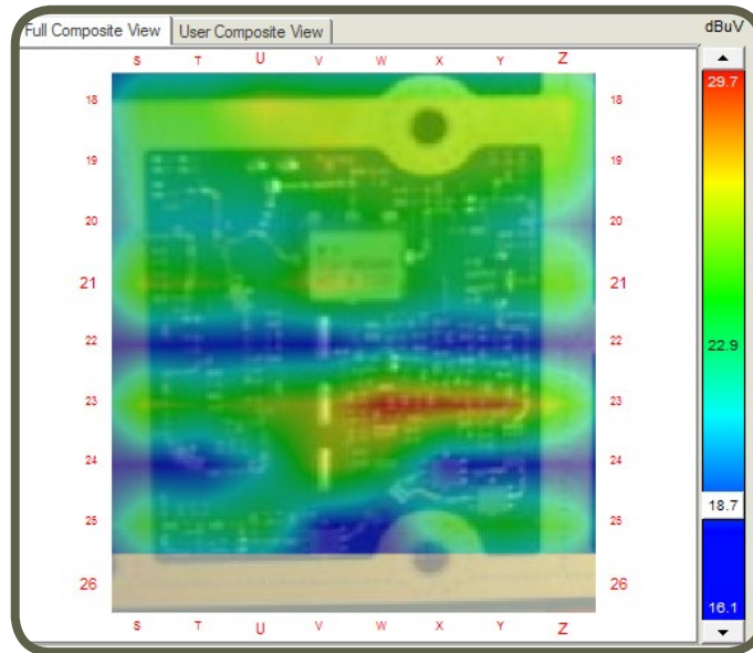
Fig. 23: Spatial Scan of the IF Chain of the Good Board Showing Strong Emissions Throughout
