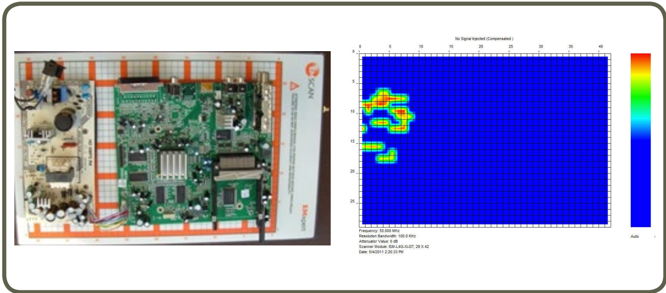
Fig. 14: EMxpert spatial scan at 50MHz with no noise injection.
