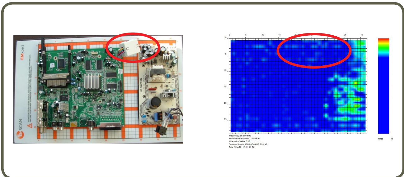
Fig. 3: The same board and test setup as before. A filter was added and the board re-tested, demonstrating that the filter eliminated the noise.
