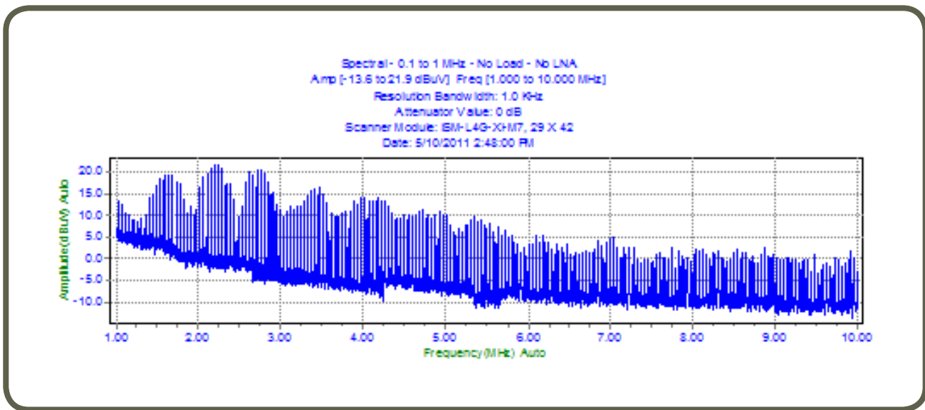
Fig. 18: Spectral scan of the broadband noise from a power supply.
