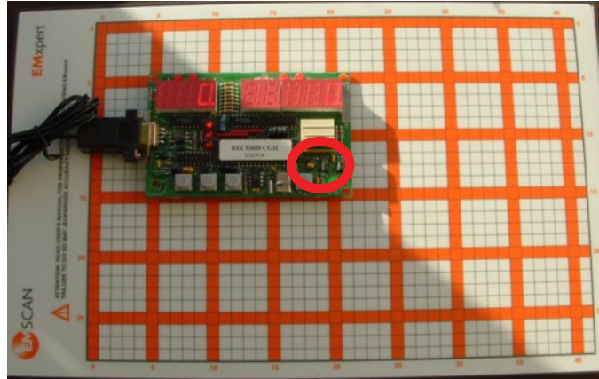
Fig. 11: Taximeter PCB positioned on the patented scanner and tested at 11.06 MHz. The test measures noise without and then with a capacitor added (location in red circle)
