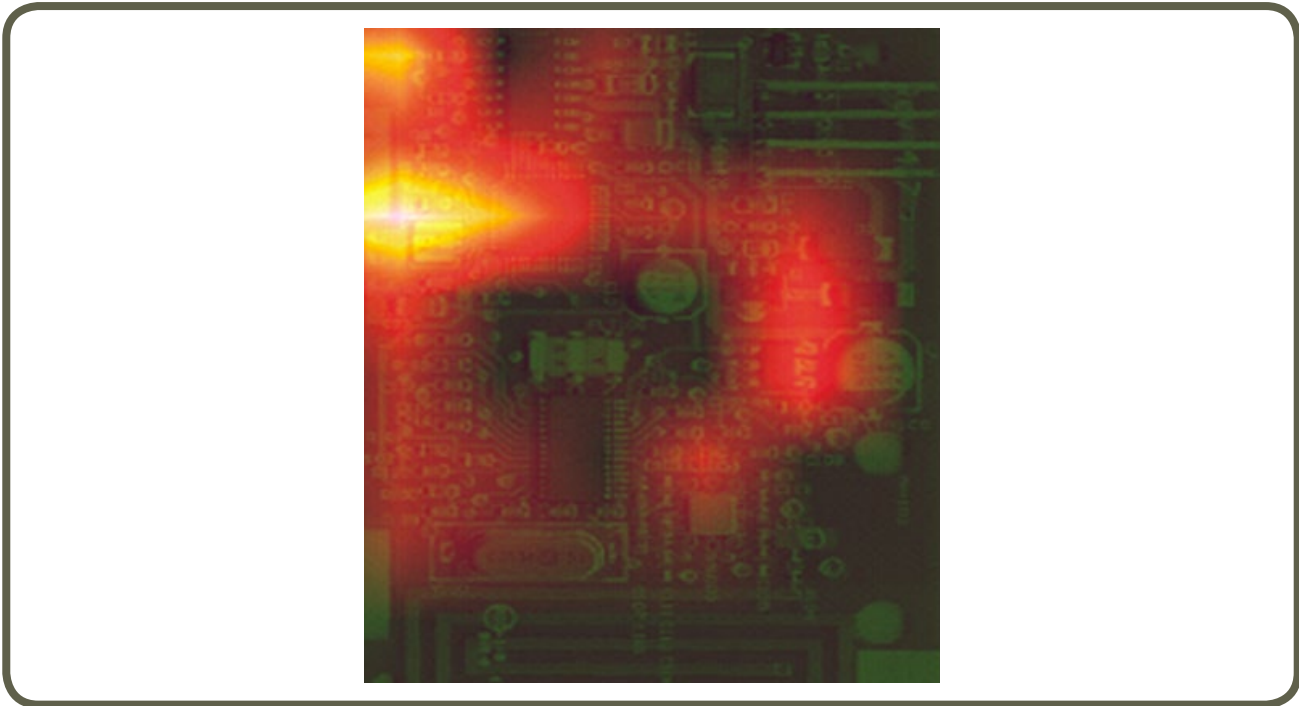
Fig. 10: EMxpert spatial scan showing low level noise coupling onto a connector at the top right.
