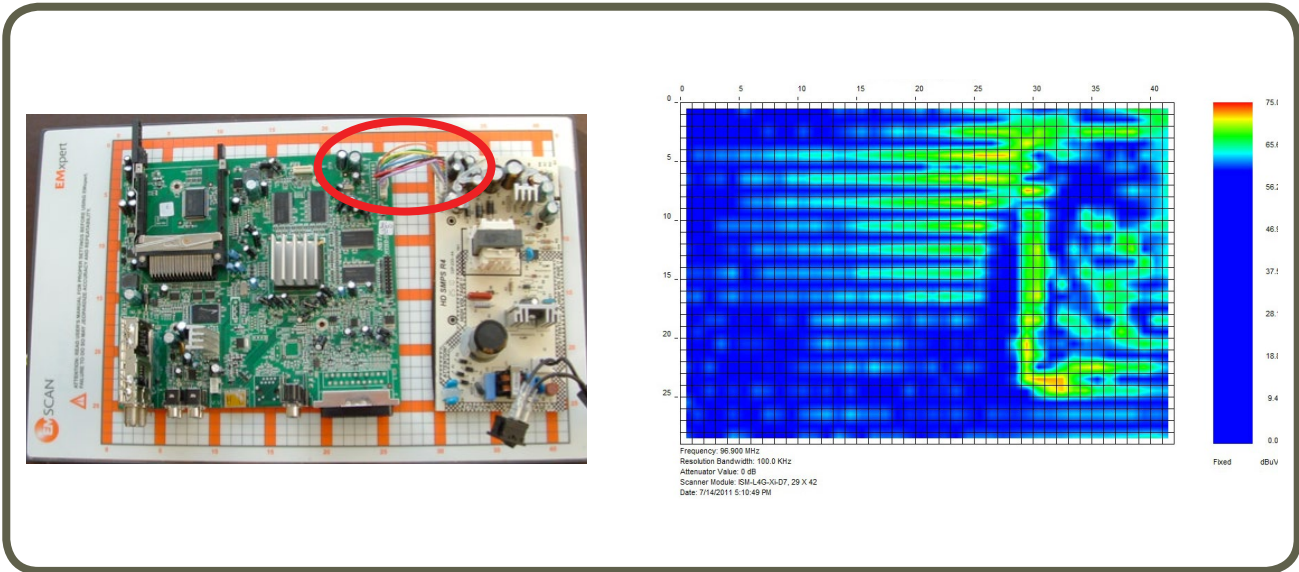
Fig. 1: Satellite Receiver Board positioned on patented scanner. Unfiltered connection to power supply circled in red.
