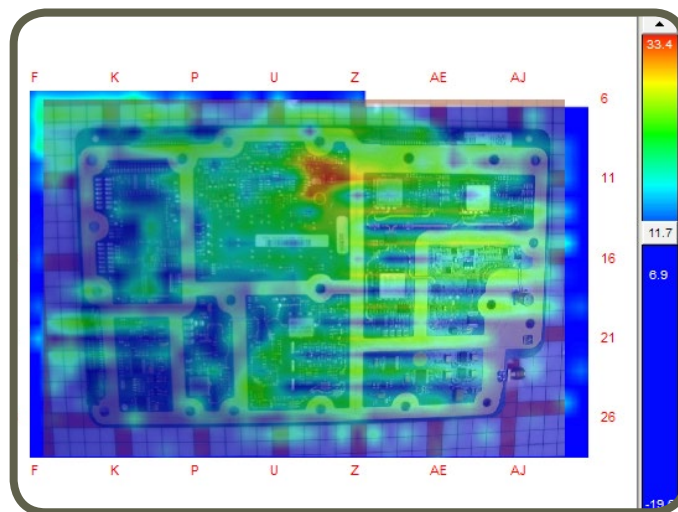
Fig. 21: Spatial Scan of the Good Board at the IF frequency
