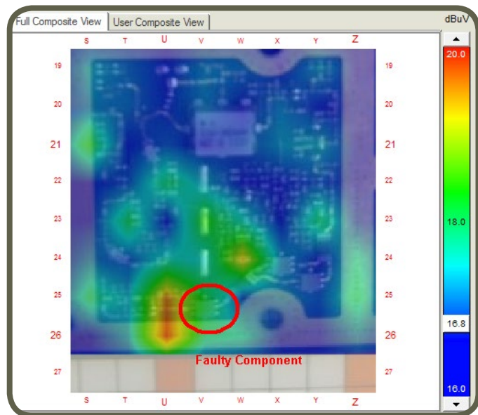
Fig. 24: Spatial Scan of the Bad Board at the IF Frequency
