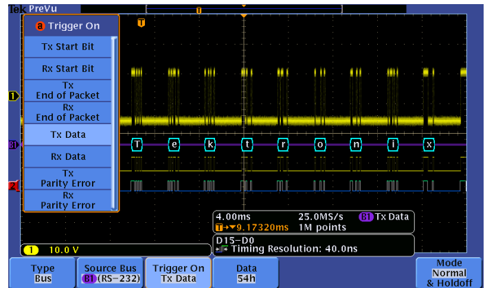
Capture – Triggering on a specific transmit data packet going across an RS-232 bus. A complete set of triggers, including triggers for specific serial packet content, ensures you quickly capture your event of interest.
