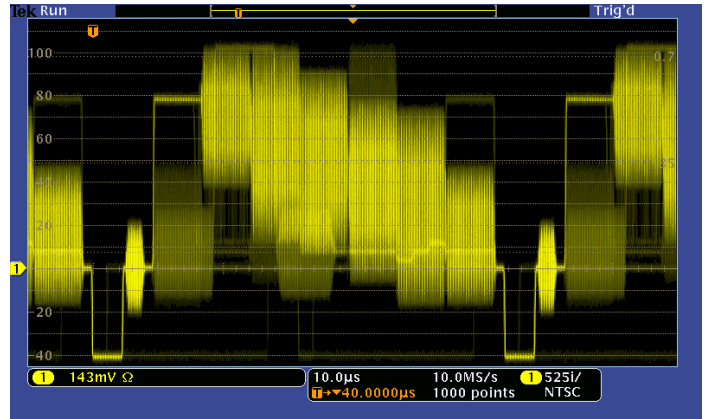
Viewing an NTSC video signal. Notice the intensity-graded view provided by the MDO's ability to represent time, amplitude, and distribution over time.
