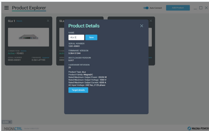
Product Details View product ratings, firmware version and hardware revision. Assign a pseudonym to the product, allowing it to be easily distinguished for multi-product control in the Dashboard Panel.
