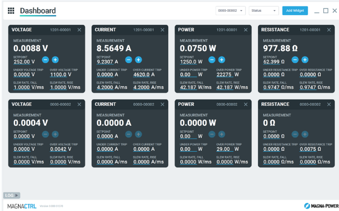
Dashboard Panel Add and remove widgets from multiple connected Magna-Power products, simultaneously, to build a dashboard using parameters and controls that are important for the specific user. Easily drag and drop widgets to organize the Dashboard.
