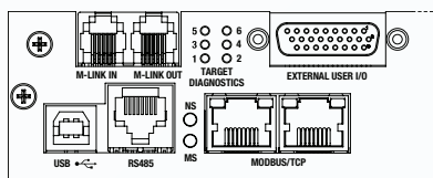
Rear communication interfaces with Modbus-TCP (+MTCP) option.
