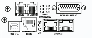
Rear communication interfaces with EtherCAT (+ECAT) option.
