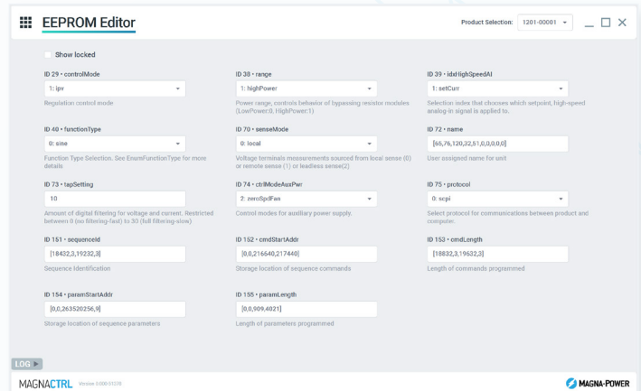
EEPROM Editor Panel Allow Magna-Power applications and support technicians to look behind-the-scenes at the product's configuration parameters using the EEPROM Editor.
