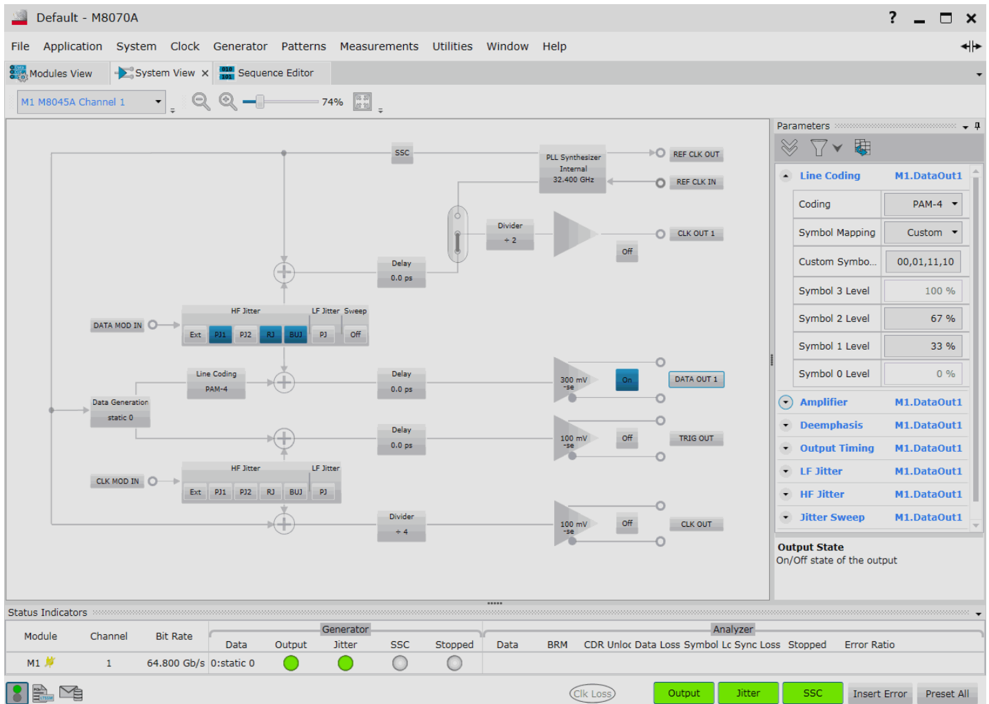
Figure 15. The graphical user interface offers multiple views that can be defined by the user. This example shows the preliminary system view on the left side and the pattern generator data output with the PAM-4 coding and level linearity parameters at the right.
