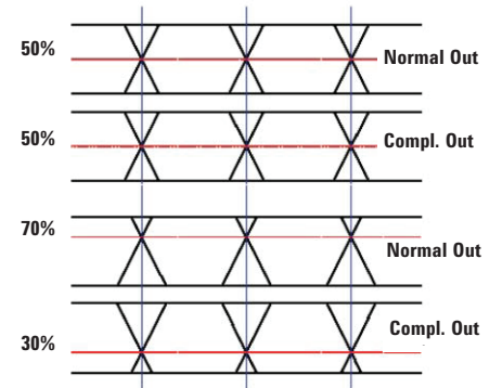
Figure 1. Variable crossover
