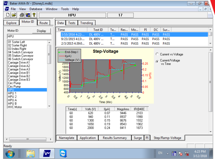
DC step voltage test results screen
