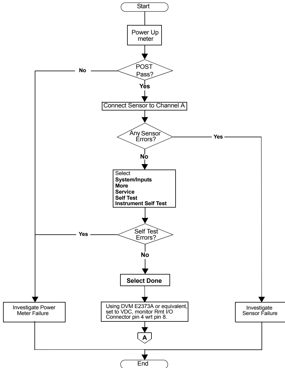
Figure 6-3 Troubleshooting Guide - TTL Output 2
