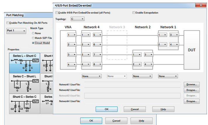
Figure 13. Fixture simulator
