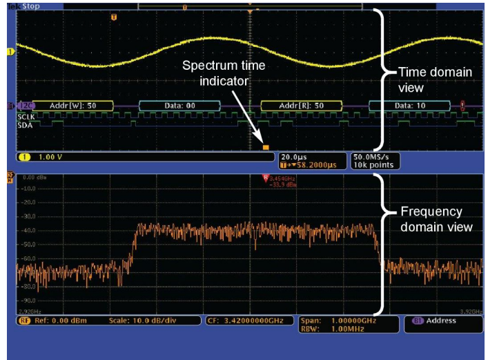
The upper half of the MDO4000B Series display shows the Time Domain view of the analog and digital channels, while the lower half shows the Frequency Domain view of the spectrum analyzer channel. The orange bar - Spectrum Time - shows the period of time used to calculate the RF spectrum.
