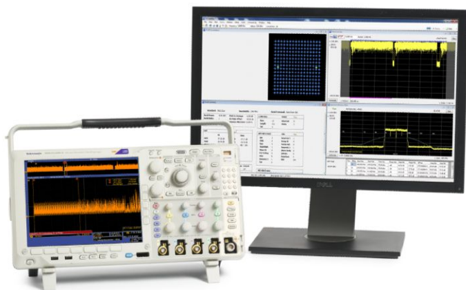
MDO4000B paired with SignalVu-PC to analyze 802.11ac modulation.
