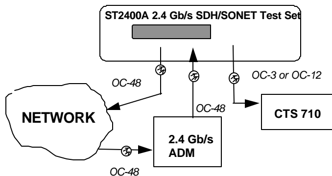
Figure 2-12. ST2400A Passive Monitoring
