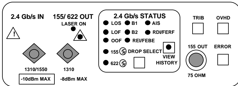
Figure 2-6. Receiver Front Panel
