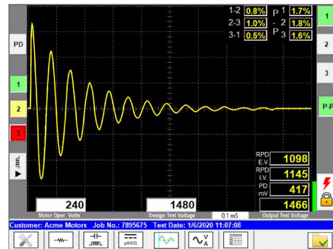
Surge Test
