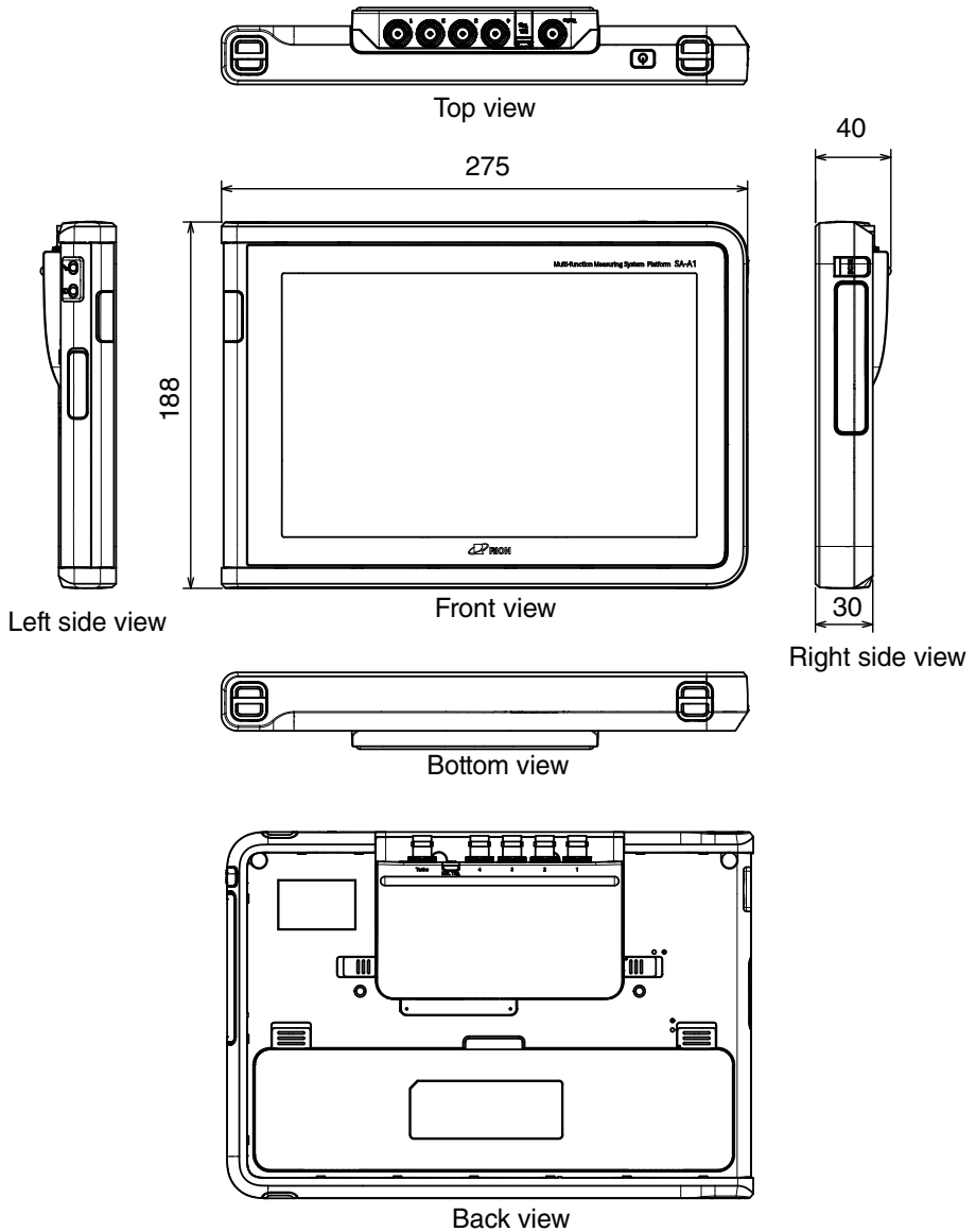
Dimensional Drawings
