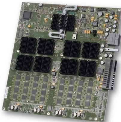
Acquisition board.
