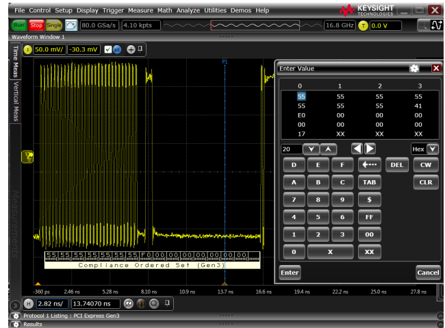
V-Series' hardware serial trigger finds a PCI Express Gen 3 compliance ordered set symbol that is 130-bit long (PCIe Gen 3 uses 128b/130b encoding).
