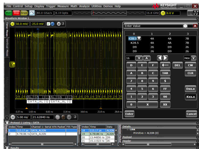
The V-Series' 8b/10b hardware triggers at 16 "K" and "D" symbols of the SATA signal. The software protocol decoder further decodes the symbols into higher-level data packets such as the SATA ALIGN packets.
