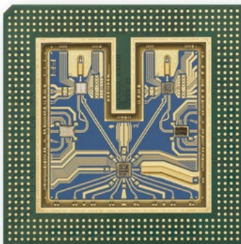
Front-end multi-chip module.
