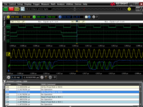
DDR3 protocol decode and write command trigger.
