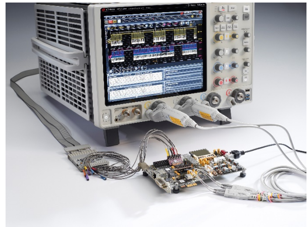
DDR3 test setup with mixed signal oscilloscope.
