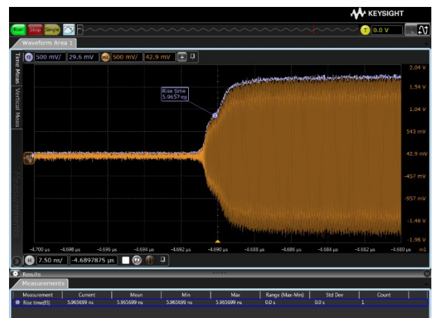
Envelope detection of signal burst.
