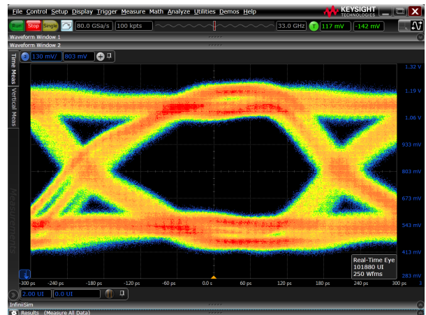
DDR3 write data burst eye-diagram analysis.
