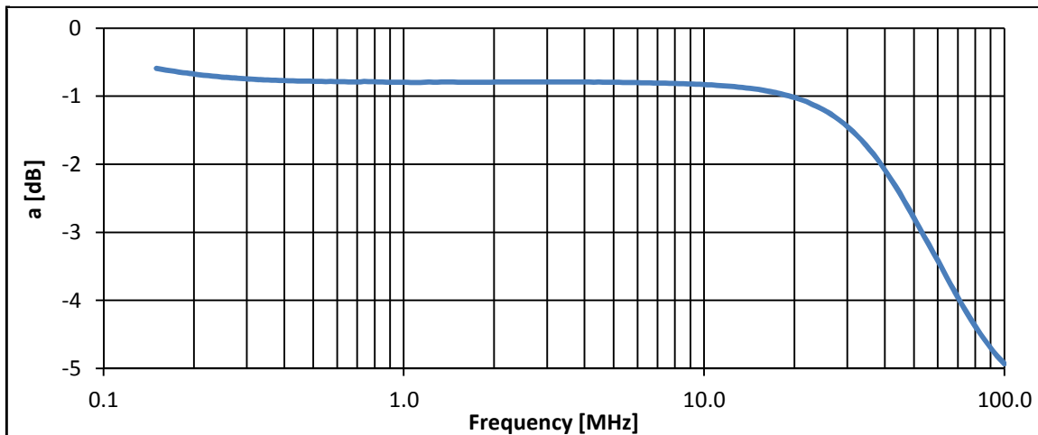
Decoupling Factor (TOSM / ABCD Transformation)
