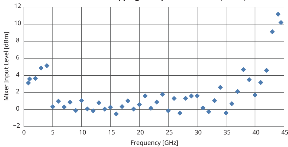
Nominal ADC Clipping vs. Input Mixer Level (meas.)
