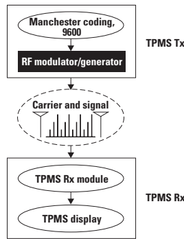
Figure 1: TPMS Functionality Action Flow
