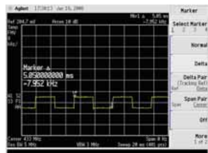
Figure 3: Data bit on ESA4402B
