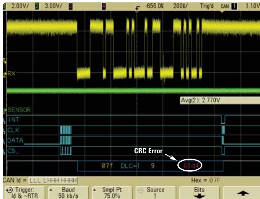
Figure 4: Random errors observed in CAN decode while triggering on data frame ID: 07F HEX
