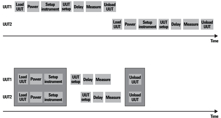
Figure 7: Multi-up testing of two or more UUTs
