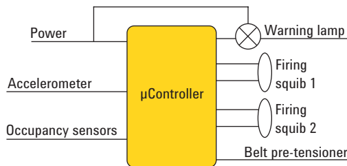
Figure 1: Centralized airbag system
