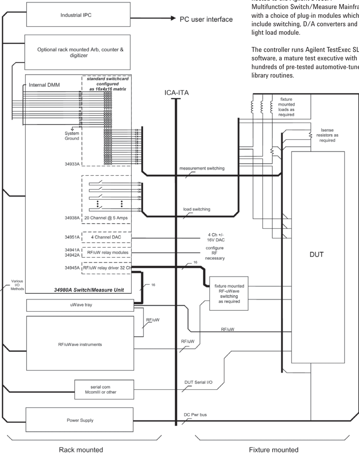
Figure 4: System Block Diagram
