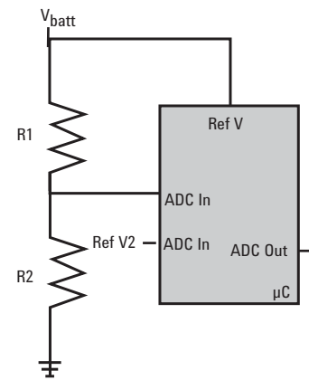
Figure 5: Measuring battery voltage with two reference voltages
