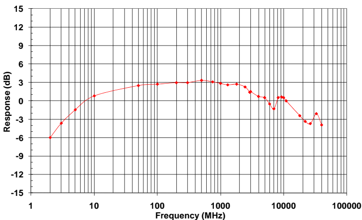
FL7040 Typical Uncalibrated Frequency Response
