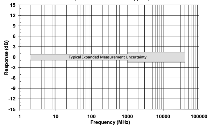
FL7040 Typical Calibrated Frequency Response (with correction factors applied)
