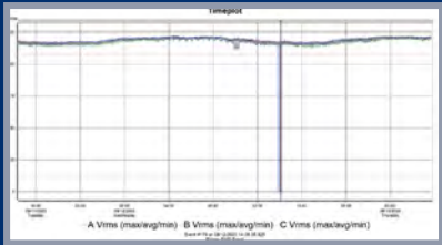
Voltage Trends
