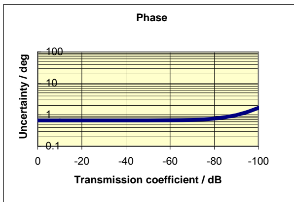
Diagram: Typical accuracy of transmission magnitude and transmission phase measurements of the R&S®ZVA50 and R&S®ZVA67 in the frequency range 700 MHz to 24 GHz.
