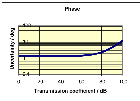
Diagram: Typical accuracy of transmission magnitude and transmission phase measurements of the R&S®ZVA50 and R&S®ZVA67 in the frequency range 24 GHz to 50 GHz.
