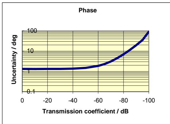
Diagram: Typical accuracy of transmission magnitude and transmission phase measurements of the R&S®ZVA50 and R&S®ZVA67 in the frequency range 10 MHz to 700 MHz.
