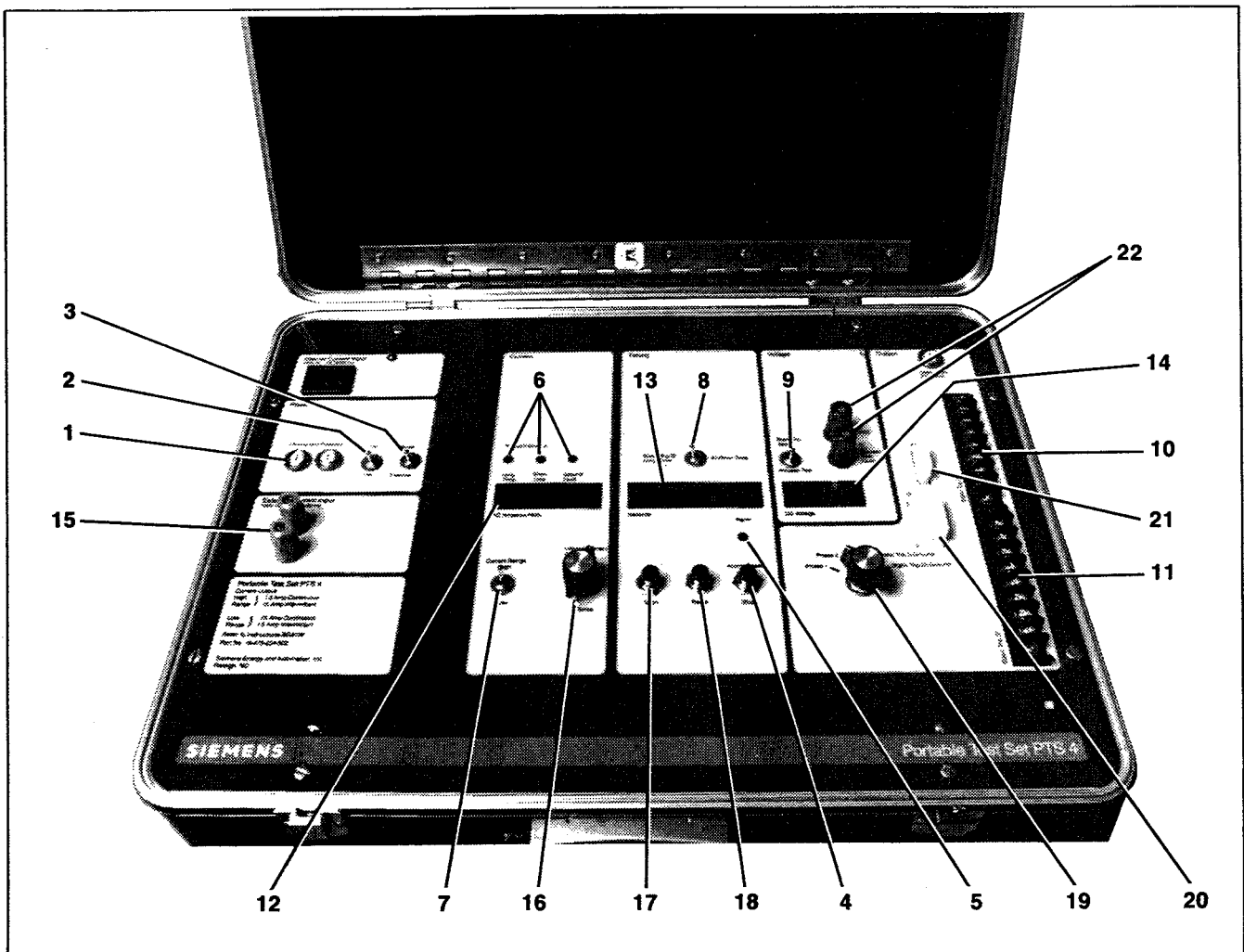
Figure 3. Control Panel
