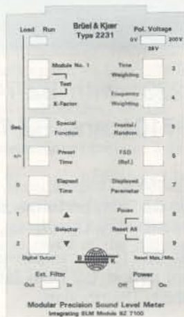
Fig. 1. Frontplate for Application Module BZ7100
