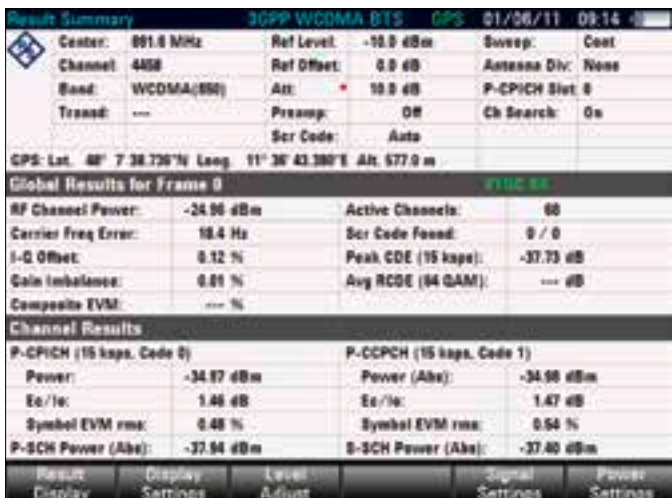
Analysis of a 3GPP WCDMA transmit signal with the R&S®FSH-K44 option.
