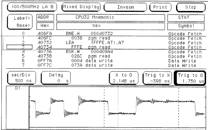
Mixed Display using the HP 16550A and HP 16532A
