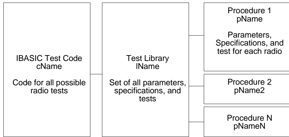
Figure 40 TESTS Subsystem File Relationship
