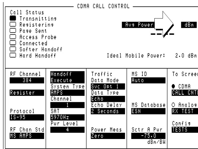
Figure 2 Units-of-Measure Field
