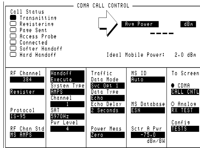
Figure 4 One-of-Many Field
