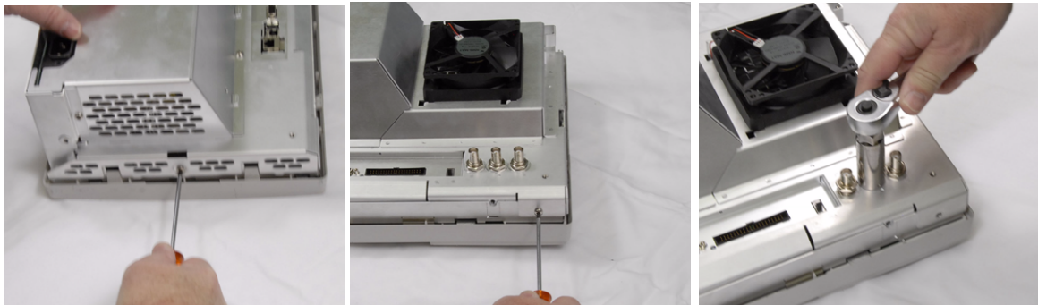
Figure 19 Removing the rear deck assembly
