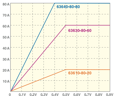
Low Voltage & V-I Curve Operating Characteristics (Typical) of 63600 Series : Model 63640/ 63630/ 63610
