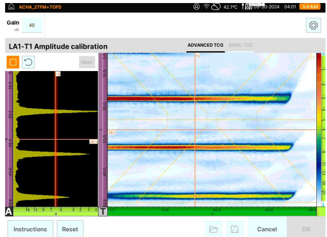
Figure 2: Calibration wizard.
