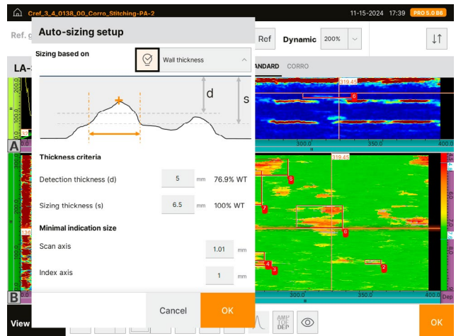
Figure 3: Automatic corrosion sizing
