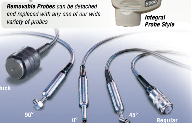
Cabled Probe Style
