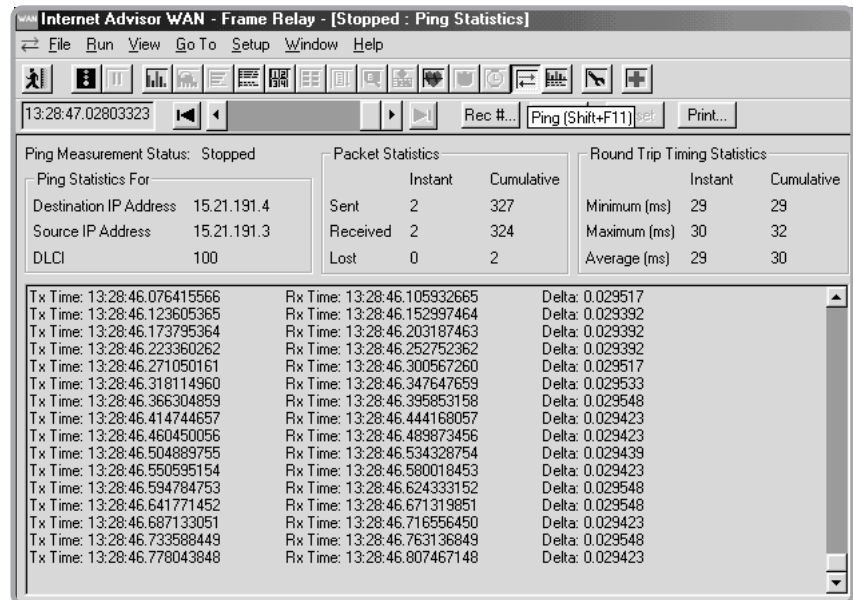
Figure 14: PING measurement.
