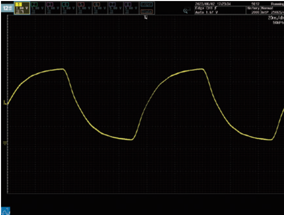
At 20 MHz
