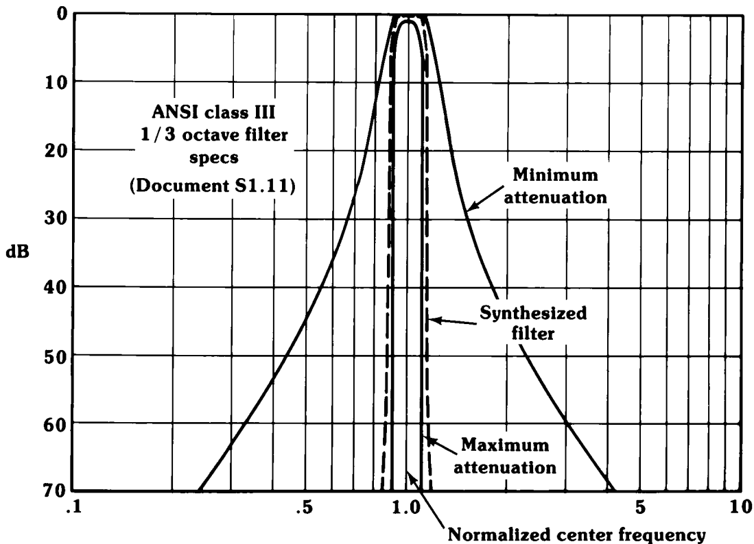
Figure 4. Filter #12
