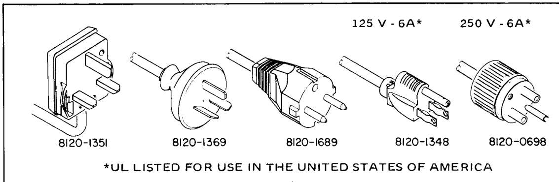
Figure 2-2. Power Cables.
