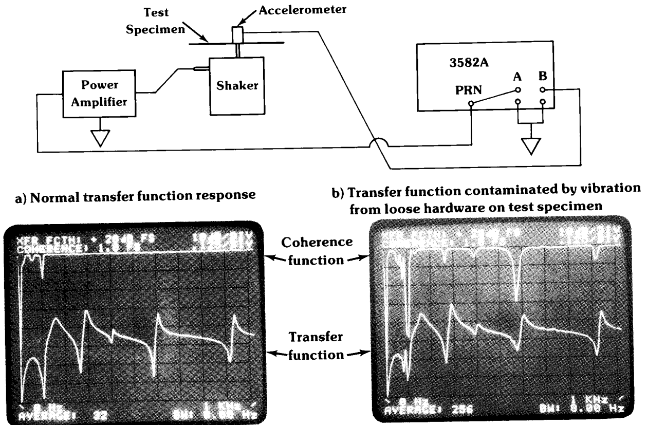
Vibration spectrum of 5" x 7" printed circuit board.
