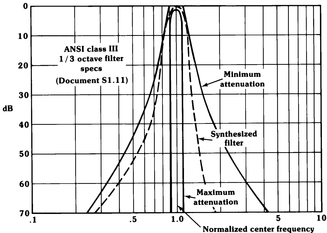
Figure 5. Filter #13
