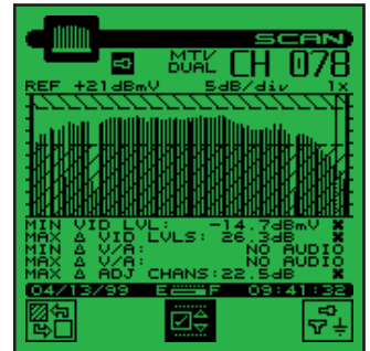
The Full Scan display shows all user-defined video carriers. The unique limit check feature quickly checks the results against user-defined analog and digital limits.
