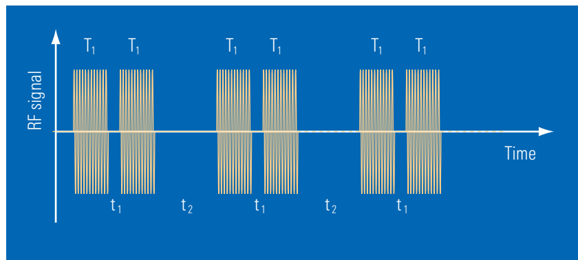
Double pulses
