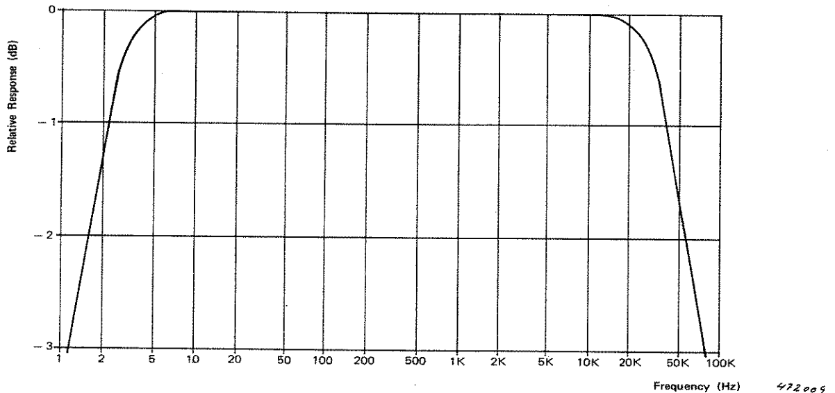
Fig.4.4. Amplifier Frequency Response (10 A RMS into a 2 \Omega load)
