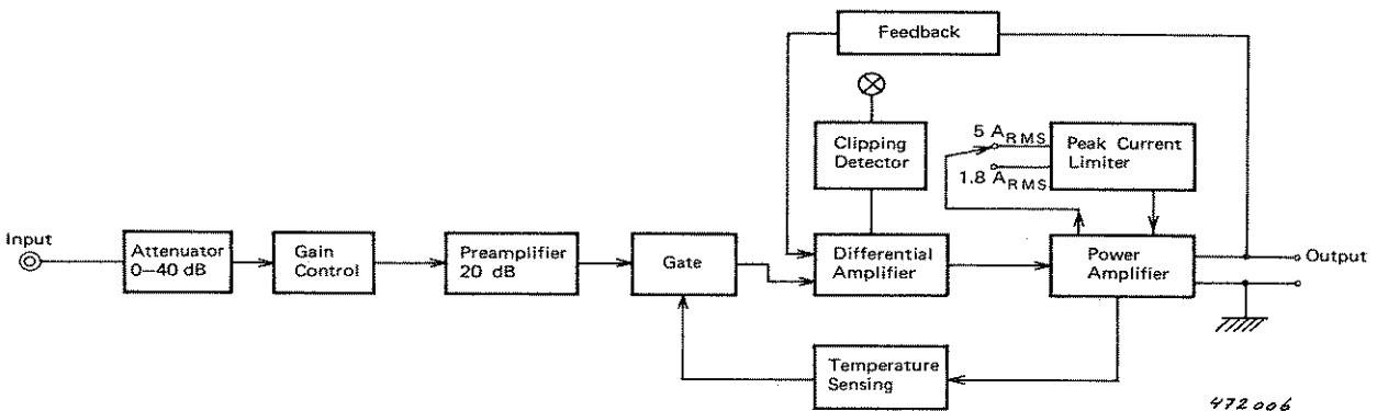
Fig.4.1. Block Diagram of 2706
