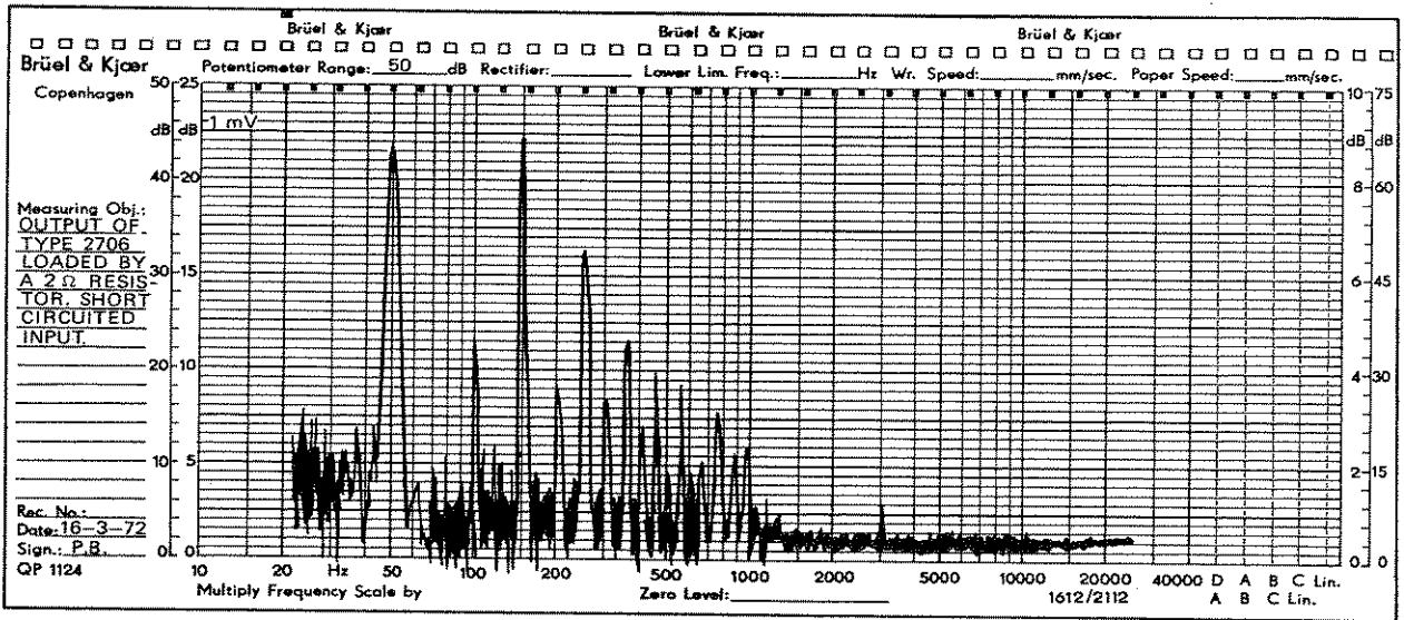
Fig.4.6. Narrow band Frequency analysis of noise and hum. Short circuited input
