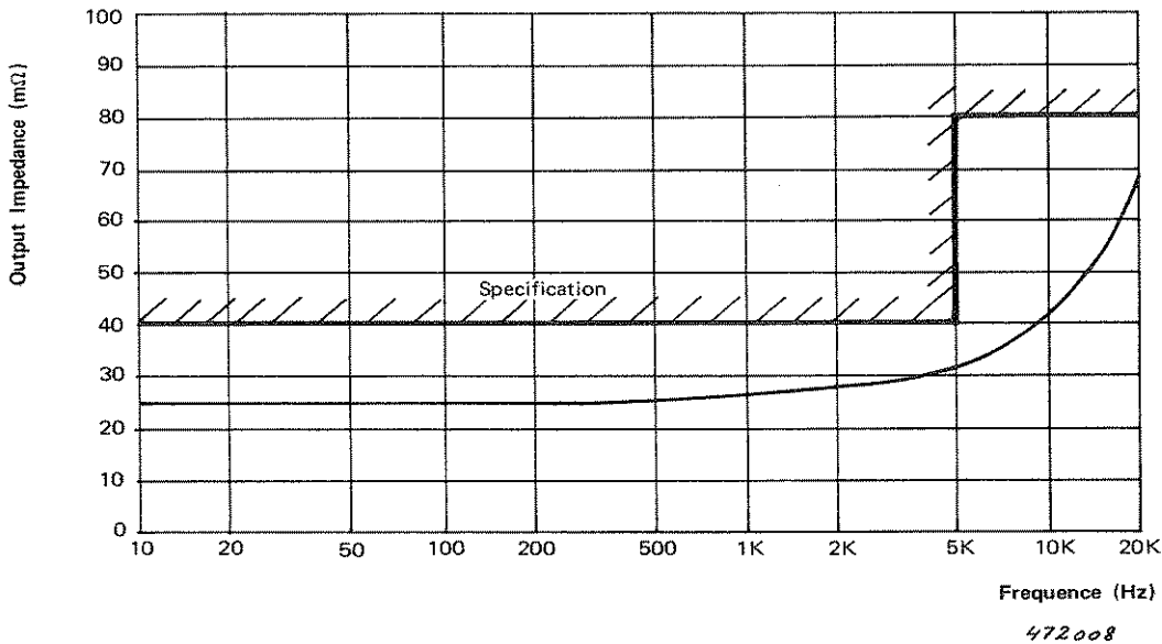
Fig.4.5. Output Impedance
