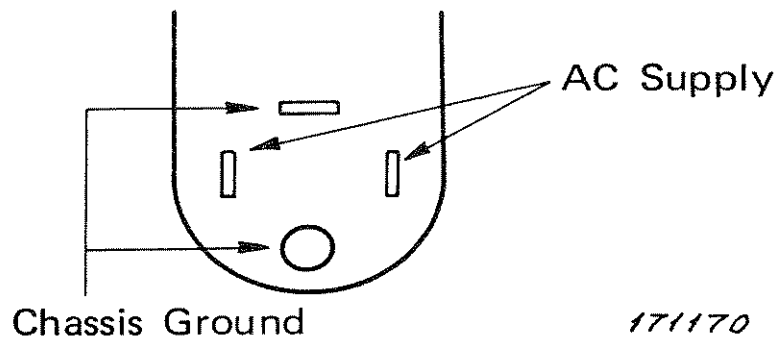
Fig.2.3. AC Power Socket
