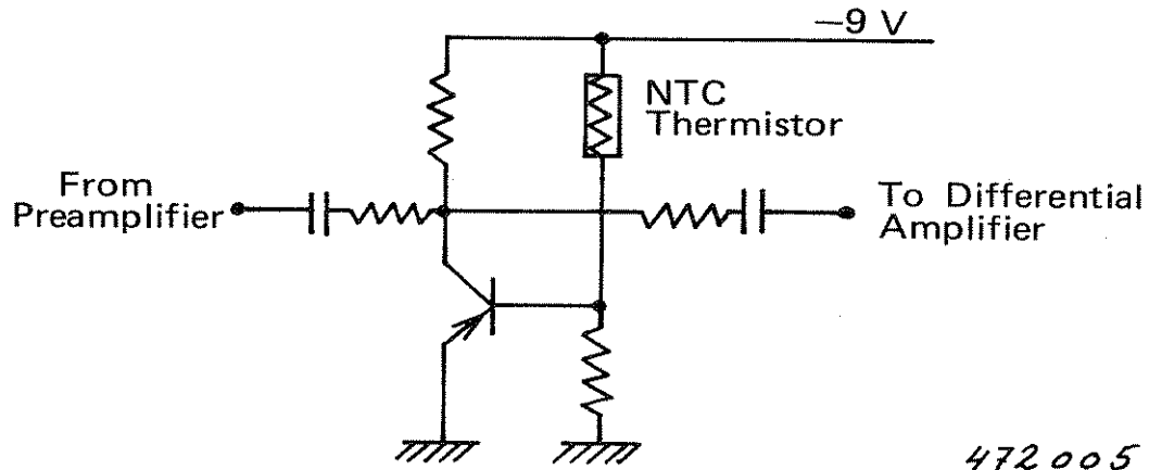
Fig.4.2. Temperature sensitive gating circuit of 2706
