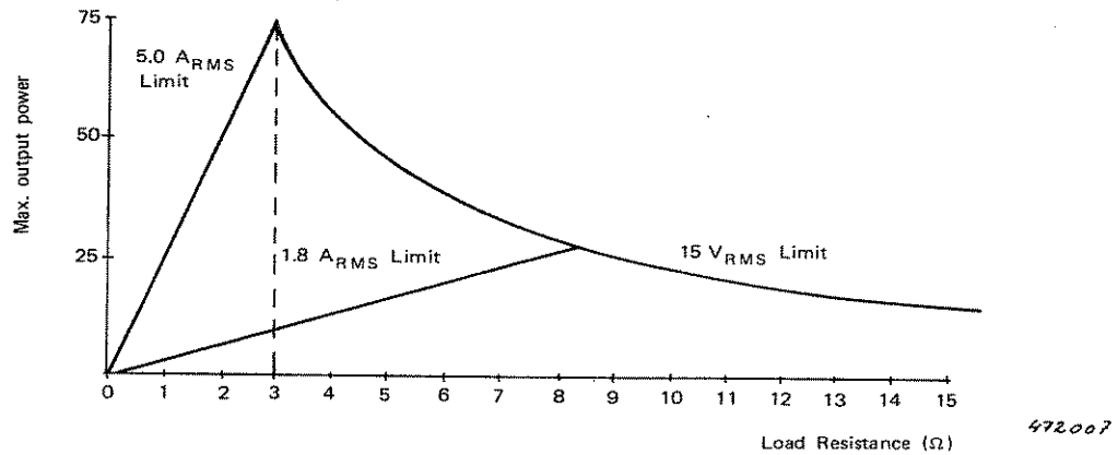
Fig.4.3. Maximum Output Power for both current limits
