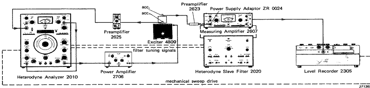
Fig.5.2. Example of Vibration Testing set-up
