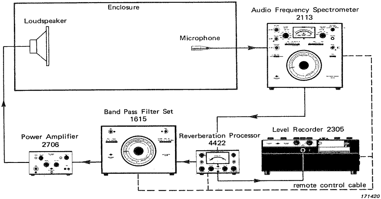
Fig.5.3. Measurement of Reverberation Time by the Kuttruff Method
