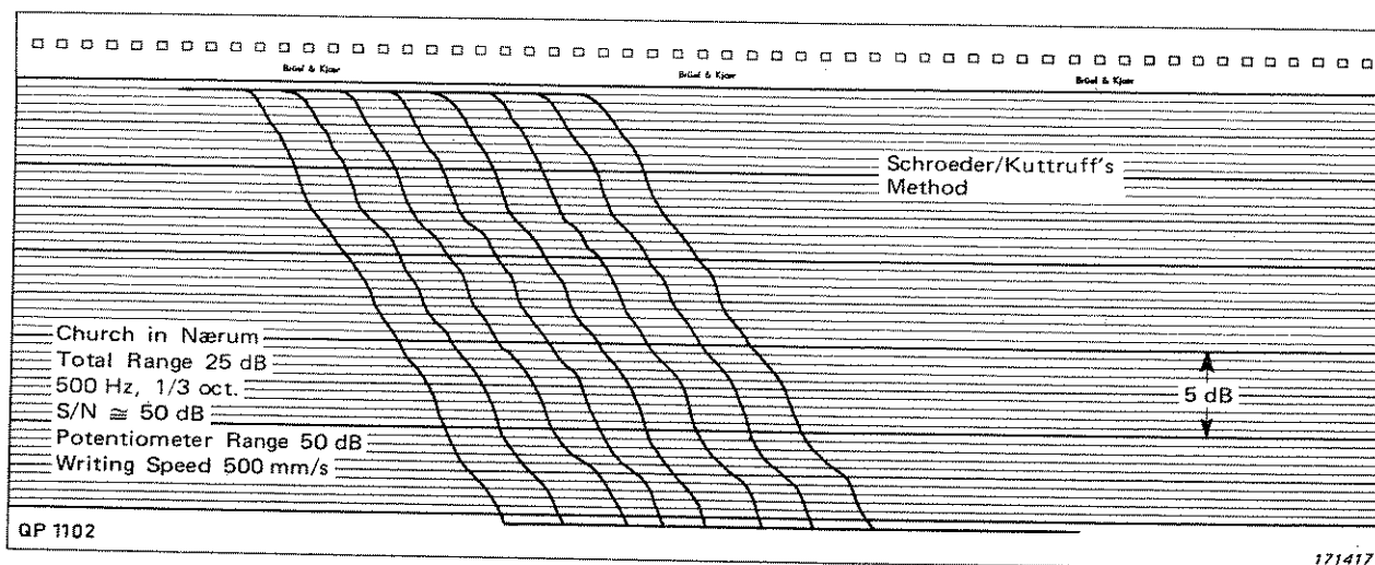
Fig.5.4. Reverberation Decay Curves, repetitive recordings
