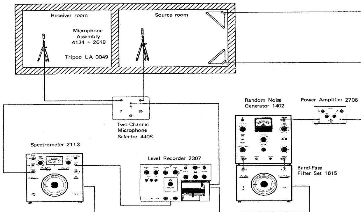
Fig.5.5. Sound Insulation measurements
