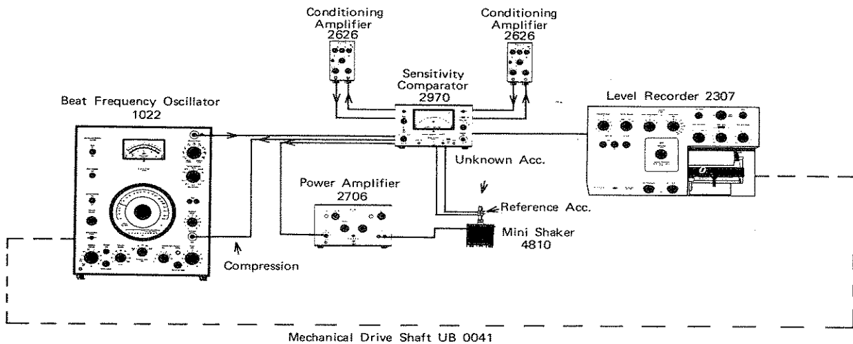
Fig.5.1. Example of Calibration set-up
