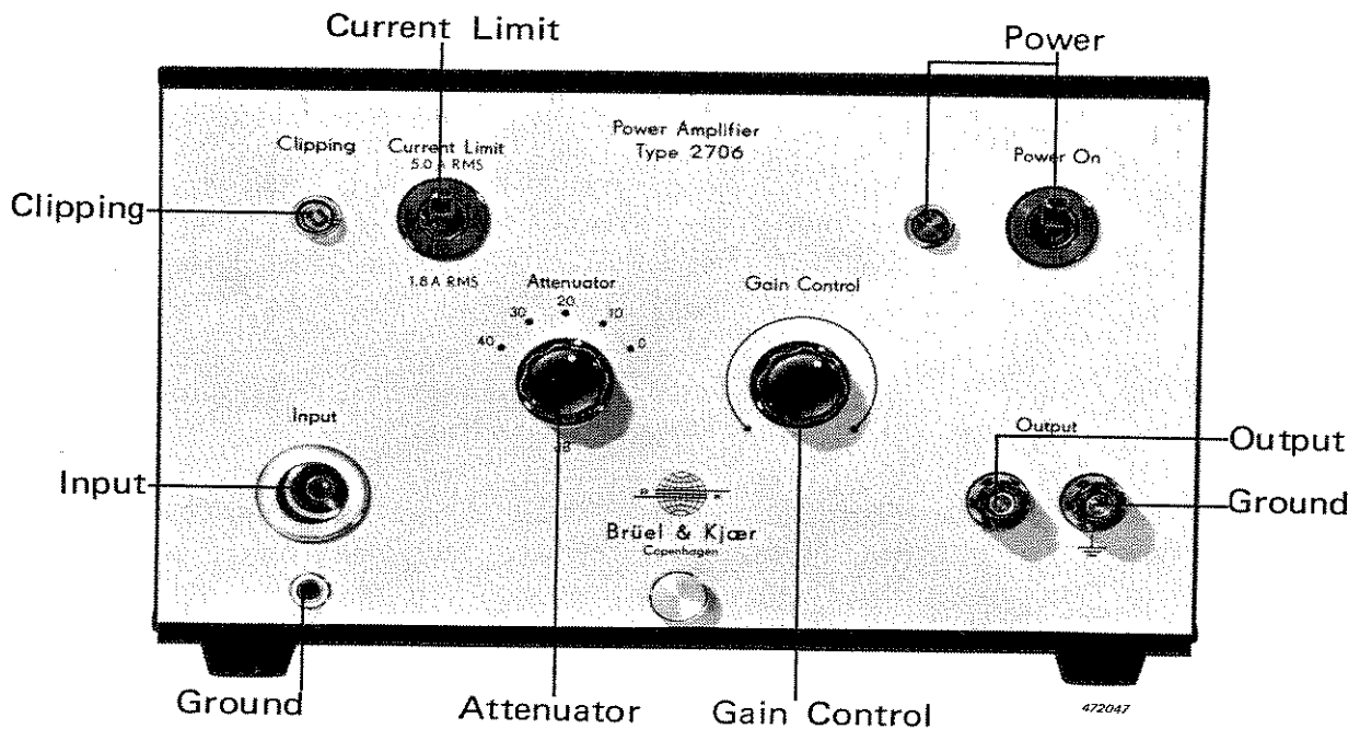
Fig.2.1. Front Panel of 2706
