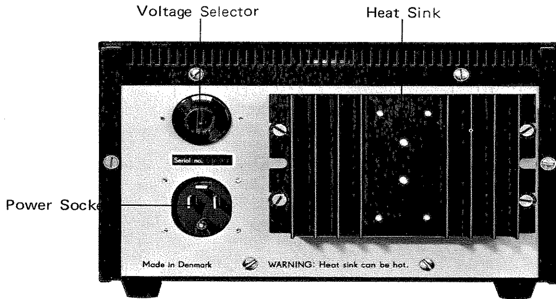
Fig.2.2. Rear Panel of 2706
