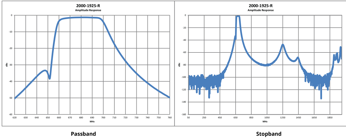
Passband
