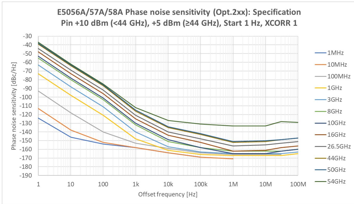
Figure 5. SSB Phase noise sensitivity (E5056A/57A/58A Option 2xx): Specification, +10 dBm (<44 GHz), +5 dBm (≥ 44 GHz) input, Auto Range OFF, Max. input level = signal level + 3 dB, start offset frequency = 1 Hz, Cross correlation factor = 1)
