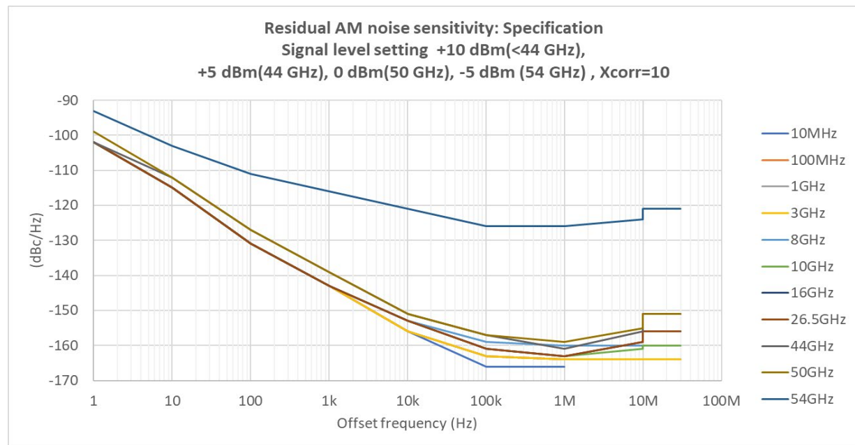
Figure 15. Residual AM phase noise sensitivity (dBc/Hz) (E5055A/56A/57A/58A): Specification, Cross correlation factor = 10, Fast XCORR mode OFF, signal level setting = +10 dBm(<44 GHz), +5 dBm(44 GHz), 0 dBm(50 GHz), -5 dBm(54 GHz), Auto range OFF, Max. input level = signal level + 3 dB, Path delay compensation 0 sec, start offset = 1 Hz 1
