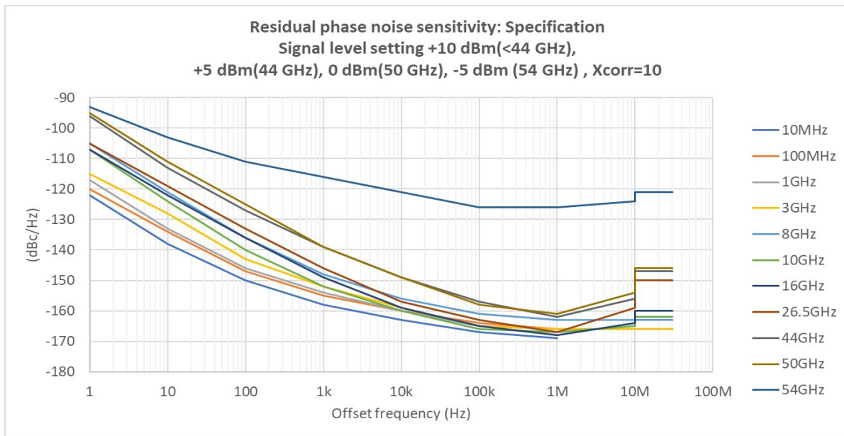
Figure 13. Residual phase noise sensitivity (dBc/Hz) (E5055A/56A/57A/58A): Specification, Cross correlation factor = 10, Fast XCORR mode OFF, signal level setting = +10 dBm(<44 GHz), +5 dBm(44 GHz), 0 dBm(50 GHz), -5 dBm(54 GHz), Auto range OFF, Max. input level = signal level + 3 dB, Path delay compensation 0 sec, start offset = 1 Hz 1
