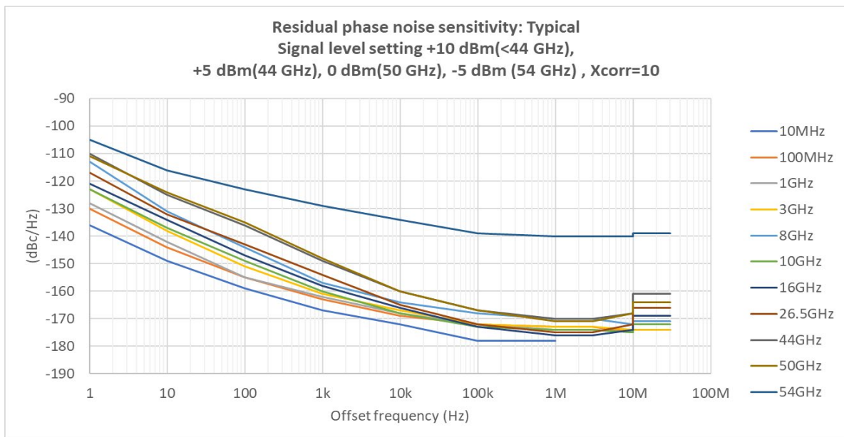
Figure 14. Residual phase noise sensitivity (dBc/Hz) (E5055A/56A/57A/58A): Typical, Cross correlation factor = 10, Fast XCORR mode OFF, signal level setting = +10 dBm(<44 GHz), +5 dBm(44 GHz), 0 dBm(50 GHz), -5 dBm(54 GHz), Auto range ON, Path delay compensation 0 sec, start offset = 1 Hz 1
