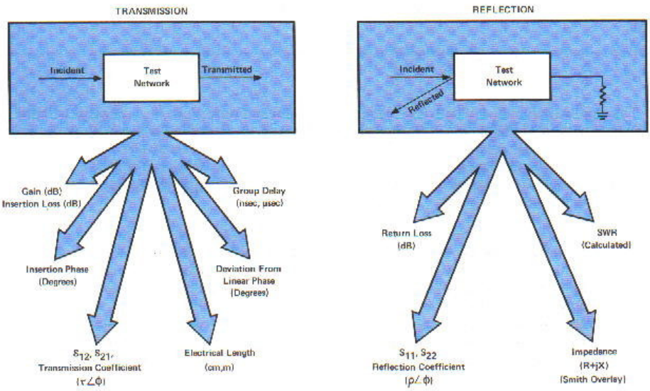
Basic 8505A Transmission and Reflection Measurements
