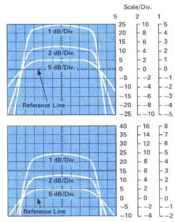
Cartesian Display
