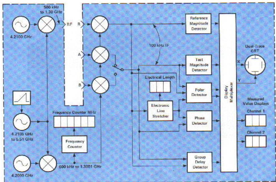
8505A Simplified Block Diagram
